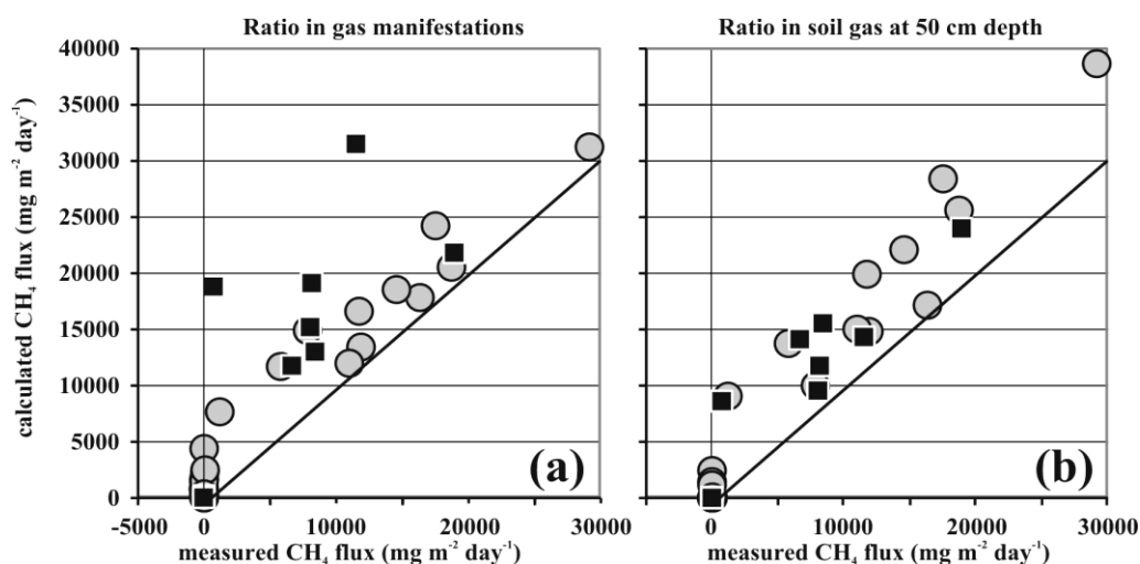
Fig. 5. Binary plot of measured vs. calculated \text{CH}_4 fluxes. (a) Fluxes calculated multiplying measured \text{CO}_2 fluxes by the \text{CO}_2/\text{CH}_4 ratios in the main gas vents. (b) Fluxes calculated multiplying measured \text{CO}_2 fluxes by the corresponding \text{CO}_2/\text{CH}_4 ratios in the soils at 50 cm depth.
