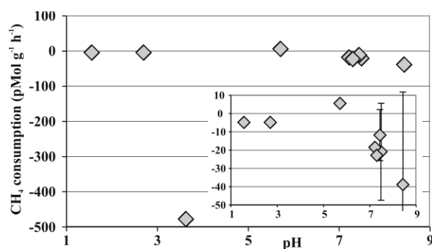
Fig. 6. Binary plot of the methane consumption rate vs. soil \text{pH}(\text{H}_2\text{O}) . Inset: same plot with enlarged y-axis. Error bar is shown for the consumption rates. Where not shown the error bar is less than the dimension of the symbol.
