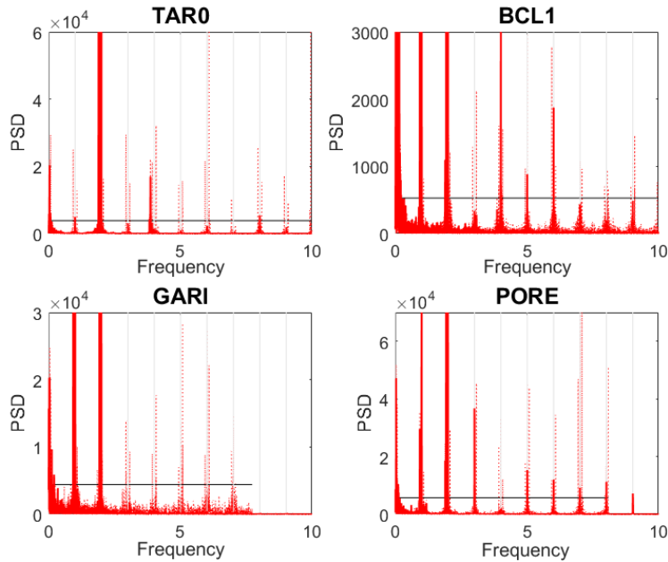
Figure 6. Spectra of Sea level data obtained from GPS data at four different stations.
