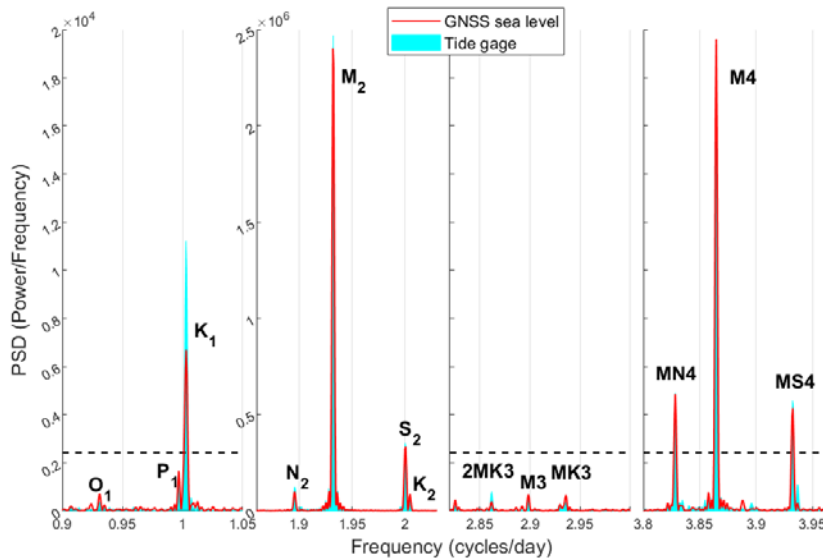
Figure 4. Spectra of one year of sea level determinations at TAR0 (Tarifa, ESP) GNSS station and tide gauge data. Tidal frequencies of the diurnal, semidiurnal, ter-diurnal and quarter diurnal constituents are shown respectively from left to right panels. Red line refers to the GNSS data and cyan line to the tide gauge data. The horizontal dashed line represents the 1% confidence level of the spectral amplitudes.
