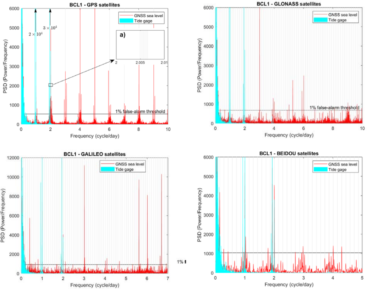
Figure 5. Spectrum of BCL1 sea level data (red) and tide gauge data (cyan) at Barcelona harbor obtained with different constellation data (GPS, GLONASS, GALILEO and BEIDOU). Grey vertical lines indicate the family of system resonances for the given constellation, the inlet a), zooming at 2 cpd, shows the fine structure of the resonance for the GPS constellation).
