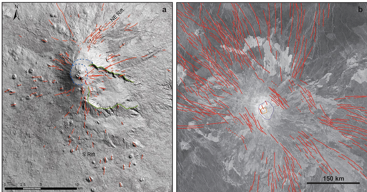
Fig. 4. Structural context of a) Mount Etna (adopted from Monaco et al., 2021 and Barreca et al., 2018 ) overlaid a hillshade DSM ( Palaseanu-Lovejoy et al., 2019 ), and b) Idunn Mons overlaid on Magellan SAR mosaic (structures adopted from López et al., 2022 ). Legend for a) Dashed blue line: buried caldera rim. Continuous green line: collapse rim. Continuous red line: volcano-rift eruptive fissures. Legend for b) Dashed blue line: flat topped summit. Dashed yellow line: summit caldera collapses. Continuous red line: volcano-rift structural lineaments. (For interpretation of the references to colour in this figure legend, the reader is referred to the web version of this article.)
