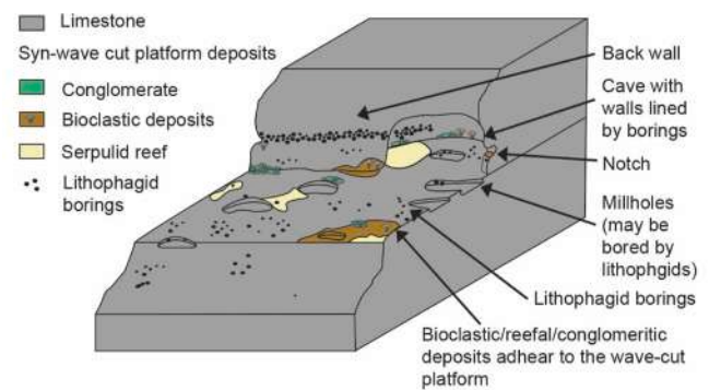
Fig. 3. Schematic diagram of the features expected on an erosional wave-cut platform, where preserved lithophagid borings and millholes indicate that erosion rates are low enough to allow for ^{36}\text{Cl} exposure dating (modified from Robertson et al., 2019).
