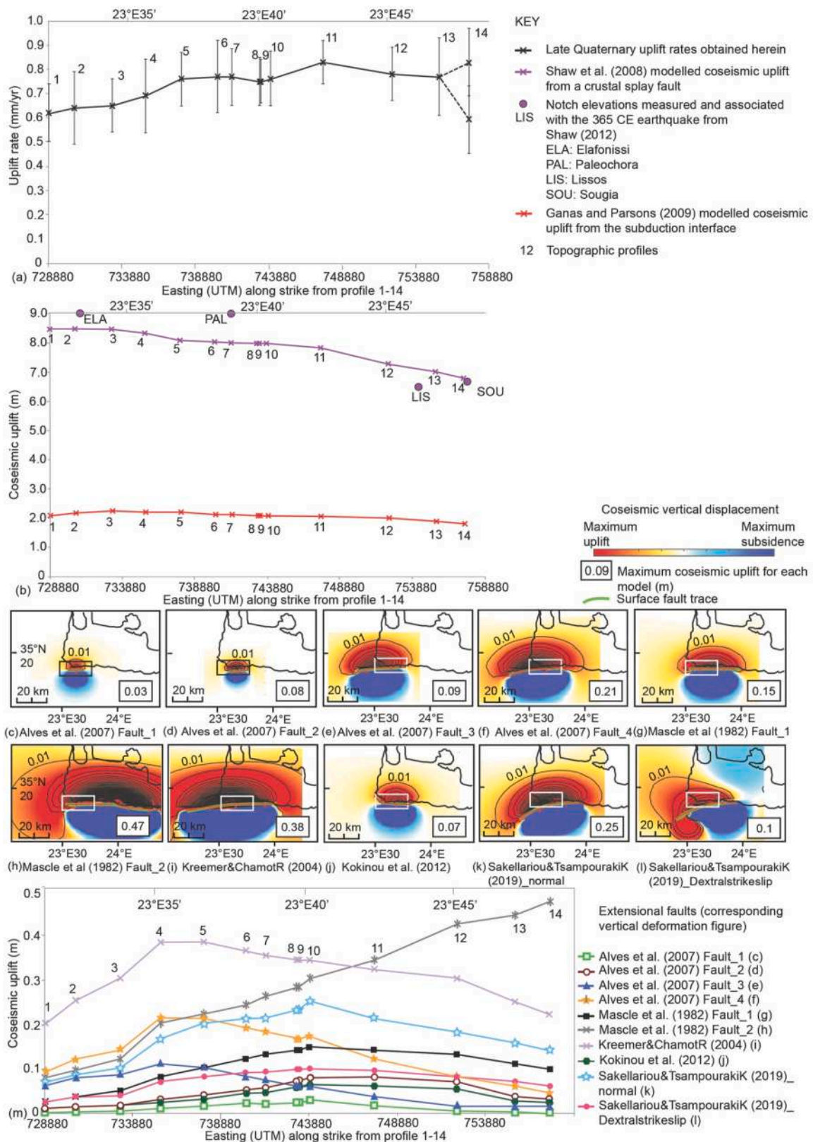
Fig. 9. (a) Late Quaternary uplift rates for P1–P14. (b) Modelled coseismic uplift from Shaw et al. (2008) and from Ganas and Parsons (2009) for earthquakes on a crustal reverse fault and the subduction interface, respectively (see Fig. 1c). (c–l) Coseismic vertical displacement modelled using Coulomb according to extensional fault traces from the studies of Alves et al. (2007), Mascle et al. (1982), Kreemer and Chamot-Rooke (2004), Kokinou et al. (2012) and Sakellariou and Tsampouraki-Kraounaki (2019) (see Table 4 for modelling values). The green line on each displacement model is the surface trace of the ruptured fault. Each contour represents 0.01 m of coseismic uplift, the maximum coseismic uplift for each model is displayed. (m) Along strike modelled coseismic vertical uplift obtained from (c–l) for fault traces.
