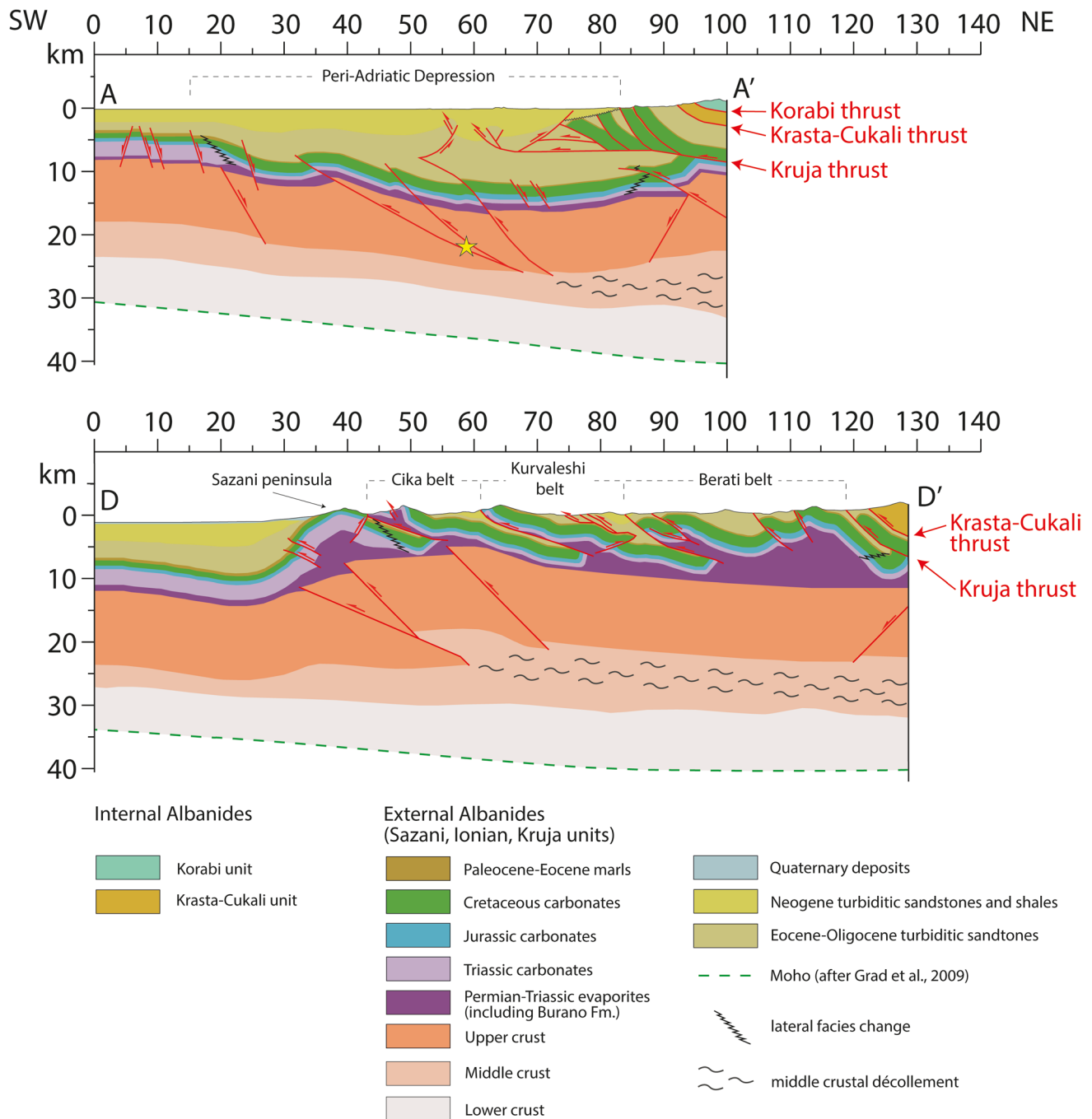
Figure 15. Crustal geological sections across the outer Albanides (section traces are located in Figure 3). No internal stratigraphy is shown for the Krasta-Cukali and Korabi tectonic units. Star shows hypocentral location of the M_w 6.4, 26 November 2019 earthquake (source: http://rcmt2.bo.ingv.it/ ; last access: 24 January 2022).
