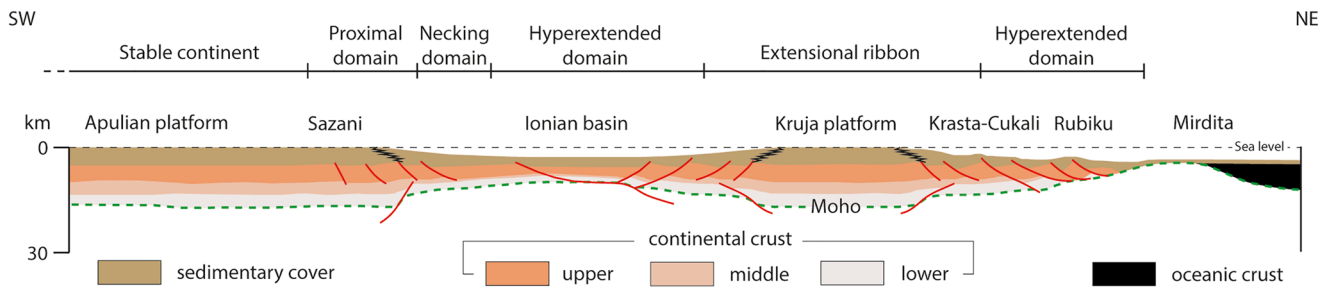
Figure 4. Schematic representation of the Early Jurassic setting of the Adria rifted continental margin in the study area.
