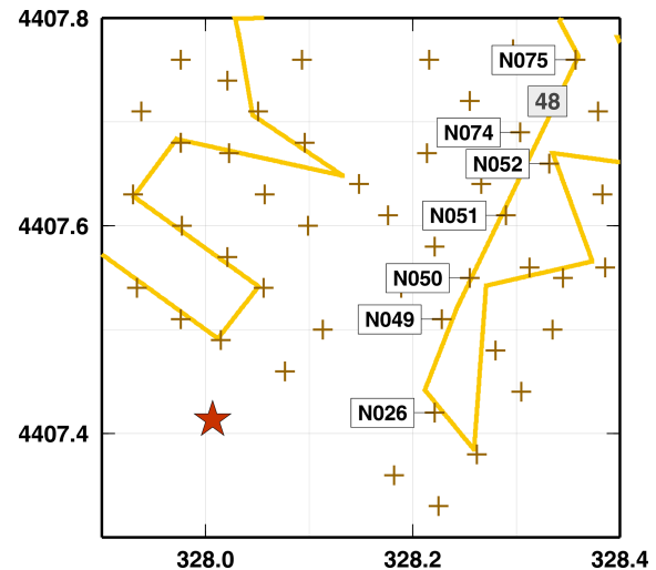
Figure A1. Map of the event, nodes and DAS segment used for retrieving P-wave delay times in the case of a local microseism. Crosses and yellow lines indicate the nodes and the DAS cable, respectively. Investigated nodes and DAS segment are labelled. A red star displays the event epicentre, as located using the geophone data and manual picking of P and S phases.
