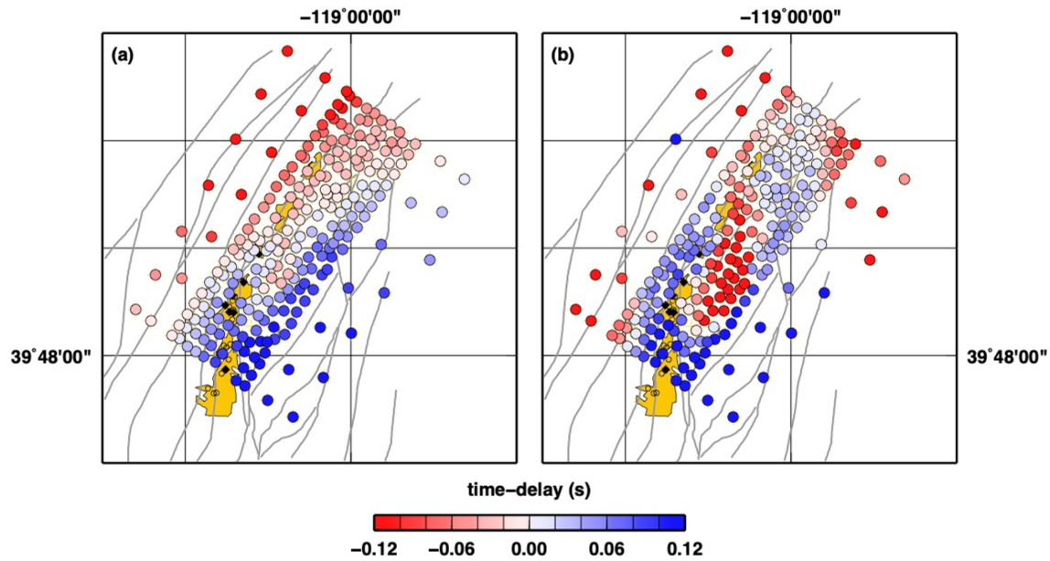
Figure 5. Maps of P-wave time delay from correlation of recordings by nodal stations. Waveforms have been filtered to 0.5–2.0 Hz: (a) vertical components; (b) north components.
