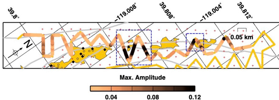
Figure 10. Amplitude analysis for all DAS segments along the northwestern side of the PoroTomo experiment (segments from 1 to 30). The dashed box indicates the area of maximum amplitude, which corresponds to the fibre cable crossing the warm ground and the area of the fumaroles/mud volcanoes.
