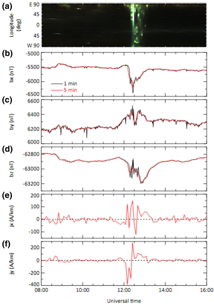
Fig. 38 (a) Keogram showing auroral activity in a zonal cross-section from the ASC. (b)–(d) Temporal variations in the geomagnetic field components measured by the dlDD magnetometer at JBS from 08:00 to 16:00 UT on 11 May 2019. The black and red lines in (b)–(d) indicate 1-min and 5-min averaged magnetic field, respectively. Panels (e)–(f) show the time plots of ionospheric currents derived from magnetic field measurements in (e) north–south and (f) east–west directions
