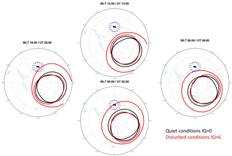
Fig. 18 Position of the poleward and equatorward boundaries of the Feldstein auroral oval for quiet ( \text{IQ}=0 , black lines) and disturbed conditions ( \text{IQ}=6 , red lines) at 12 MLT (top), 6 MLT (right), 00 MLT (bottom) and 18 MLT (left). The corresponding UT time is also reported in the figure. Black and blue dashed lines indicate the field of view at 350 km spanned by the receivers located at SANAE (black dot) and Troll (blue dot) considering an elevation angle mask of 30^{\circ}
