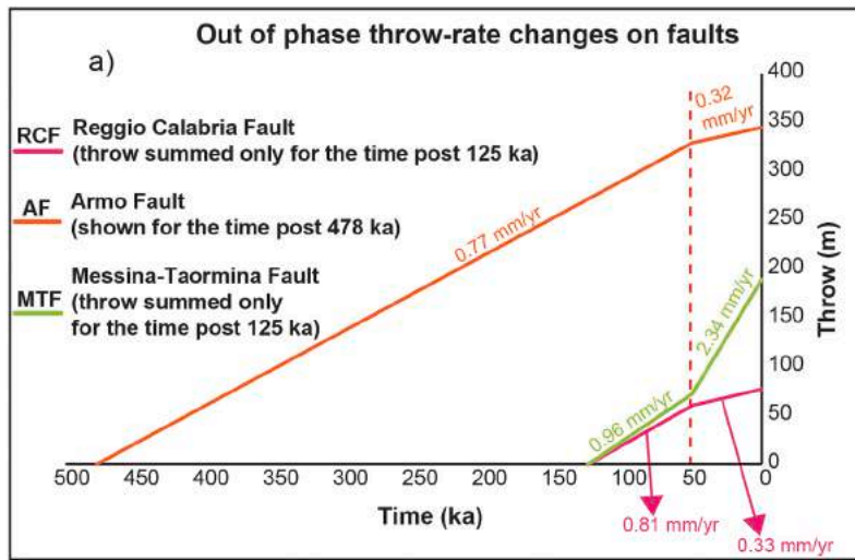
Fig. 10. (a) Throw-rates through time are shown for the Messina-Taormina Fault, Reggio Calabria Fault and Armo Fault. Changing throw rates through time have been calculated from faulted coeval marine terraces for the Reggio Calabria Fault and Armo Fault. In (b) and (c) a tectonic sketch with refined throw-rate through time, pre and post 50 ka, with horizontal extension rates from Serpelloni et al. (2010). Note that photos are from Google EarthTM (Maxar Technologies, Landsat). In (d), values of throw-rates-converted heave rates are shown, iterating different fault dip-angles for all 3 investigated faults, compared to those proposed by Serpelloni et al. (2010) using geodetic measurements. In (d), we assume that fault dip angles for all 3 investigated faults are the same because we have no information for those values. The contrast of changing throw-rates of individual faults with constant heave-rates when summed all the faults suggests that faults are interacting to maintain the regional extension rate.
