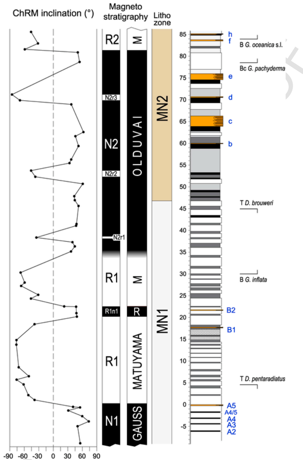
Fig. 7. Results of the paleomagnetic investigation in the “Mandorlo” section. Left: ChRM inclination values, calculated for the samples that yielded a dependable paleomagnetic result. Centre: magnetostratigraphic interpretation, with indication of Chrons formal coding (left column) and names (right). R: Reunion. Chron boundaries have been defined in correspondence to the midpoints of polarity transits, i.e., inclination = 0°. The potential Reunion Subchron (R1n1) and the short-lived intervals of reverse polarity within the Olduvai Subchron (N2r1-N2r3) have been graphically restricted to the intervals where the correlative samples are located. The stratigraphic position of relevant biohorizons is also reported (far right).
