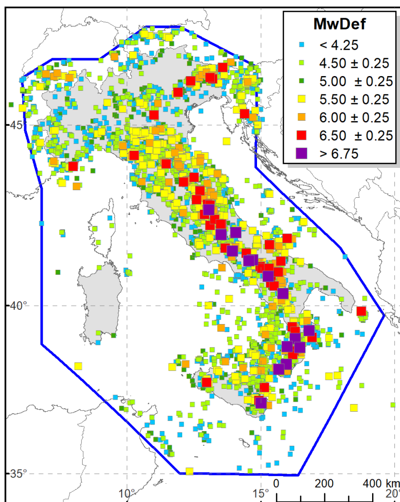
Figure 1. Map of the epicentres of the earthquakes listed in CPTI15, by M_w classes and border of the areal coverage (blue polygon).
