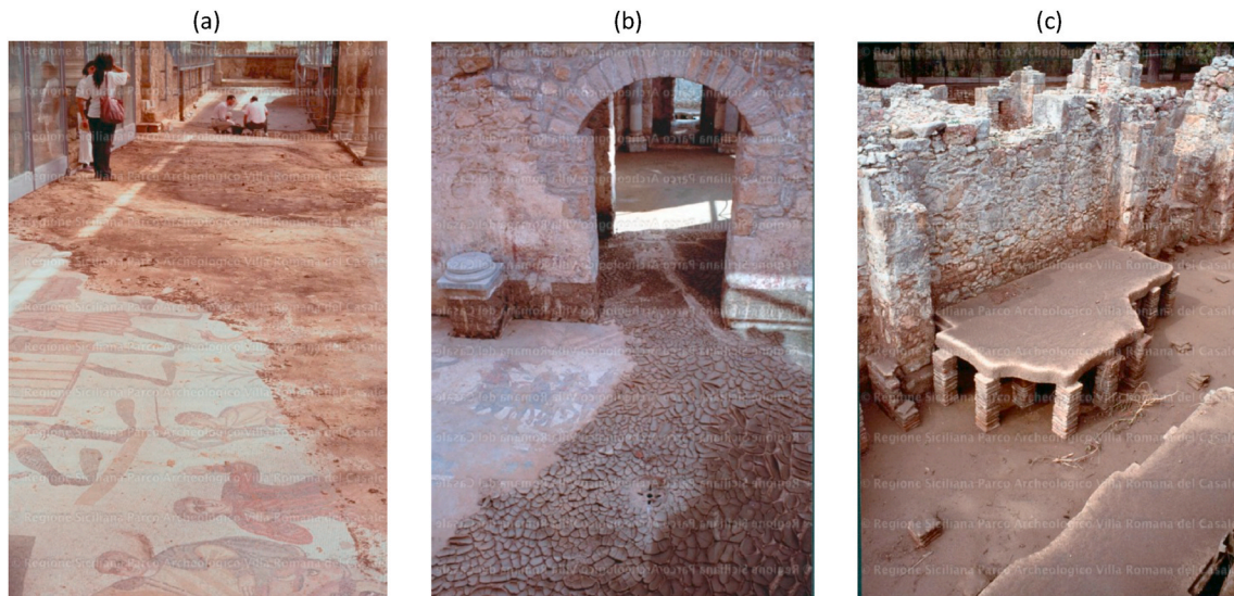
Fig. 6. Debris on the mosaics after 1991 debris flow (a): Corridoio della Grande Caccia (“Ambulatory of the Big Hunting Scene”); (b): Palestra (“Fitness room”); (c): Calidarium (“Warm room”). The absence of the floor and the bottom of the hollow space at a lower level makes the room easy to be flooded (source: www.villaromanadelcasale.it ).
