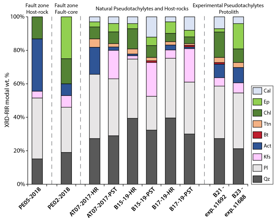
Figure 8. Mineralogical compositions (XRD semi-quantitative analysis) of the Bolfin Fault Zone host-rock and fault-core, natural pseudotachylytes (including their host rocks) and of the protolith sheared with SHIVA to produce experimental pseudotachylytes (B21: chlorite-rich, for experiment s1692, and B23: epidote-rich for experiment s1688). Cal, calcite; Ep, epidote; Chl, chlorite; Ttn, titanite; Bt, biotite; Act, actinolite; Kfs, K-feldspar; Pl, Plagioclase; Qz, Quartz.
