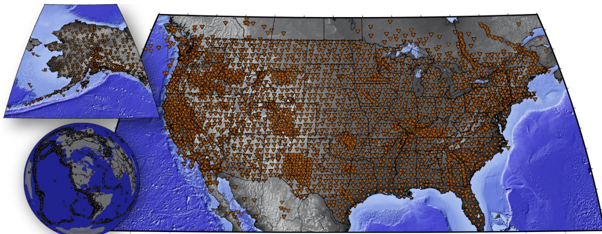
Figure 1: Location map of stations in the contiguous US and Alaska (upper inset). Lower inset depicts event coverage centered on the contiguous US.
