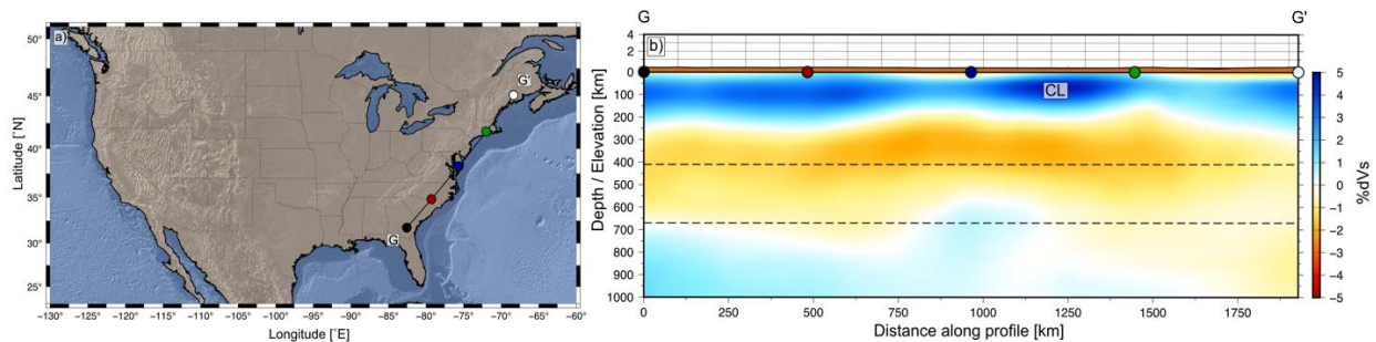
Figure 10: Cross-section through the US eastern seaboard. Panel (a) is the location map and panel (b) is the cross-section. Continental lithosphere (CL) is labeled.
