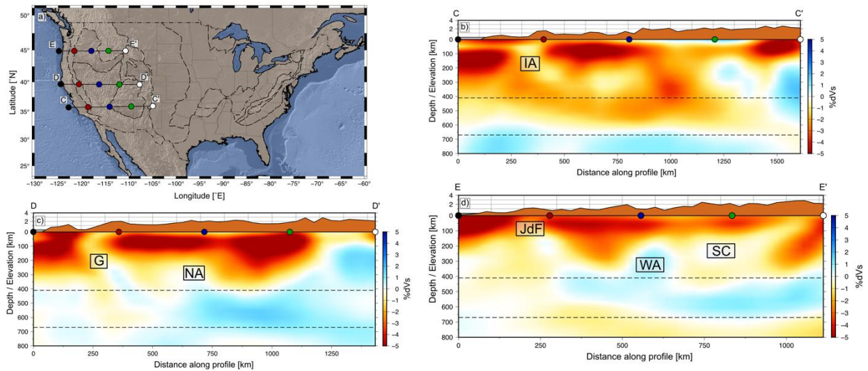
Figure 8: Illustration of reported lithospheric instabilities or stalled slabs. Labeled features include the Juan de Fuca slab (JdF), Siletzia Curtain (SC), Wallowa Anomaly (WA), Gorda slab (G), Nevada Anomaly (NA), and Isabella Anomaly (IA). Panel (a) is the location map for lines C-C', D-D', and E-E'. Asymmetrically colored dots on the lines correspond to the surface projections of the same points on the cross-sections. Dashed black lines indicate the Mantle Transition Zone at 410 km and 670 km depth. Vertical exaggeration varies with each section. Panel (b) shows the Isabella Anomaly, panel (c) crosses the Gorda plate and Nevada Anomaly (West et al. , 2009), and panel (d) goes through the Juan de Fuca slab, Wallowa Anomaly, and Siletzia Curtain (Schmandt & Humphreys, 2011).
