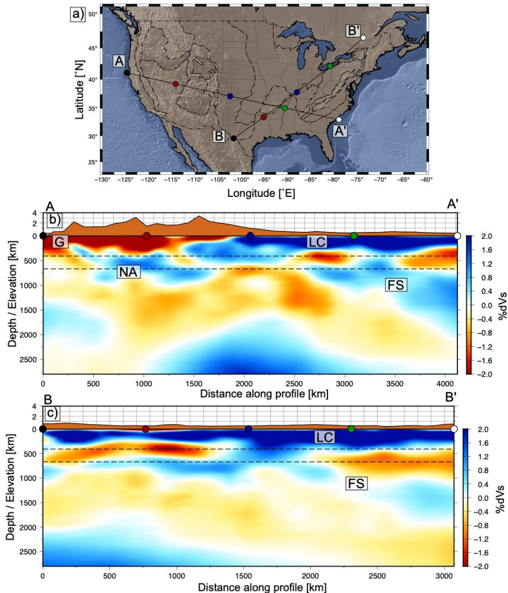
Figure 7: Cross sections along strike and dip of the Farallon system. Labeled features include the Gorda slab (G), Nevada Anomaly (NA), Laurentia Craton (LC), and Farallon Slab (FS). Dashed black lines indicate the Mantle Transition Zone at 410 km and 670 km depth. Vertical exaggeration varies with each section. Panel (a) is the location map for lines A-A' and B-B'. Asymmetrically colored dots on the lines correspond to the surface projections of the same points on the cross-sections. Panel (b) is roughly along the southern edge of the system and panel (c) is along dip of the center to eastern portion of the slab.
