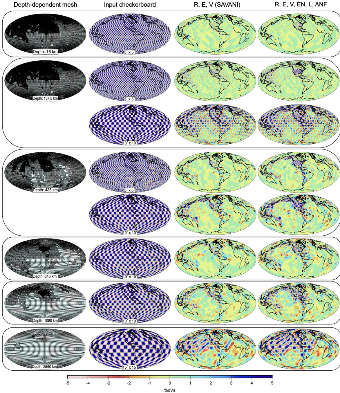
Figure 2: Global scale checkerboard resolution tests. Boxes are used to indicate common depth slices. Left hand column depicts the depth-dependent mesh centered on the Americas with the depth indicated at the bottom. Minimum size of a voxel is 0.3125^\circ \times 0.3125^\circ and maximum size is 5^\circ \times 5^\circ . Second column from the left is the input checkerboard at that depth. Radial extent of each checker is 6 layers and the thickness of each layer varies with depth: \sim 10 km through the crust, \sim 50 km through the lithosphere, and \sim 150 km through the mid to lower mantle. Third from the left is the test using only data used in Auer et al. , [2014] aside from the higher order modes from Visser et al. (2008). This data includes Ritsema et al. (2011) (R), Ekström (2011) (E), and Visser et al. , (2008) (V). Right hand column is the test for the new model including additional data from Ekström (2014, 2017) (EN), Lai et al. (2019) (L), and the Array Network Facility (ANF).
