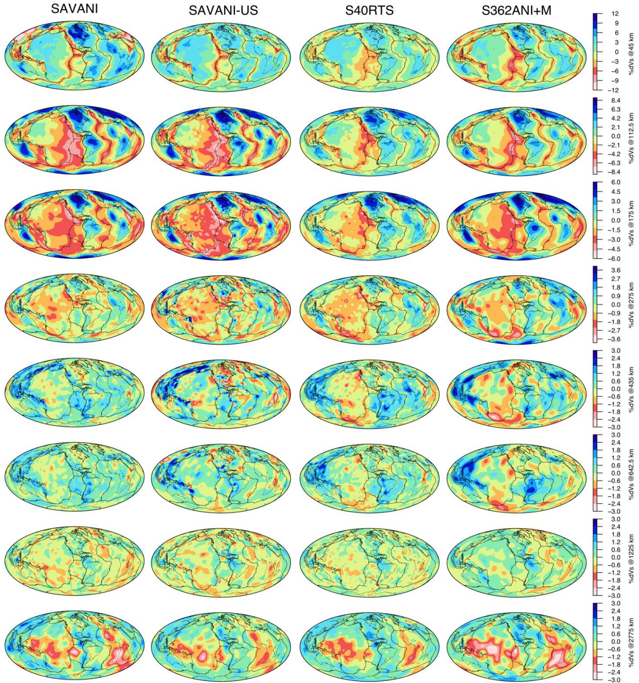
Figure 4: Map view comparison of global model isotropic shear velocity. Each column represents one model and each row is a depth slice with a common color scale indicated on the right. Left-hand column is SAVANI (Auer et al. 2014), second from left is SAVANI-US (this study) third from left is S40RTS (Ritsema et al. 2011), and the right-hand column is S362ANI+M (Moulik & Ekström, 2014).
