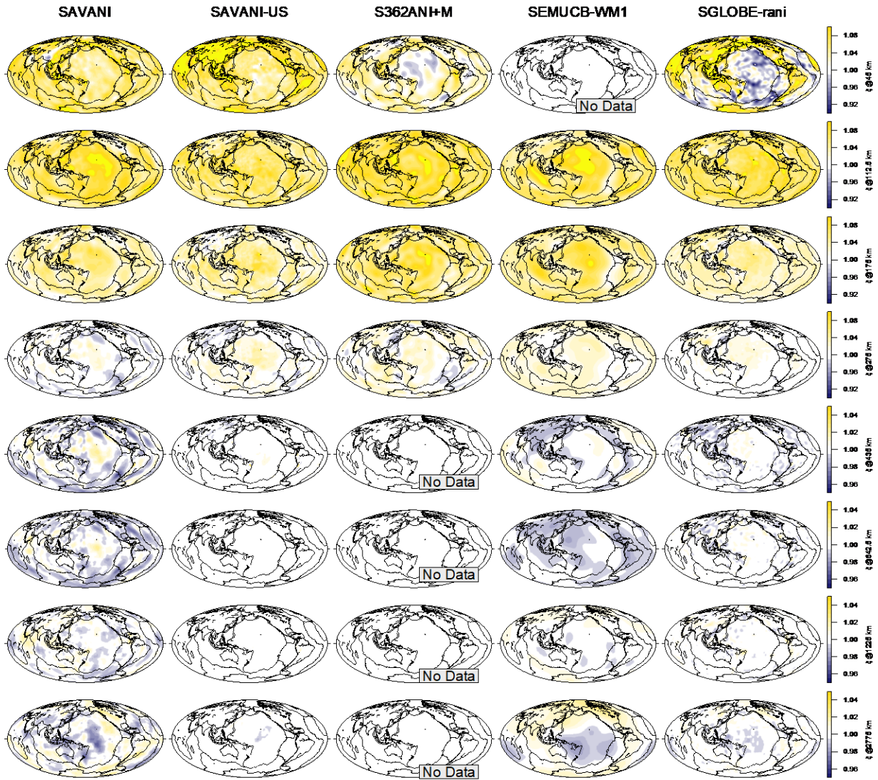
Figure 5: Map view comparison of global model radial anisotropy ( V_{sb}/V_{sv} ) 2 . Each column represents one model and each row is a depth slice with a common color scale indicated on the right. Left-hand column is SAVANI (Auer et al. , 2014), second from left is SAVANI-US (this study), center is S362ANI+M (Moulik & Ekström, 2014), the second from the right-hand column is SEMUCB-WM1 (French & Romanowicz, 2014), and the rightmost column is SGLOBE-rani (Chang et al. , 2015).
