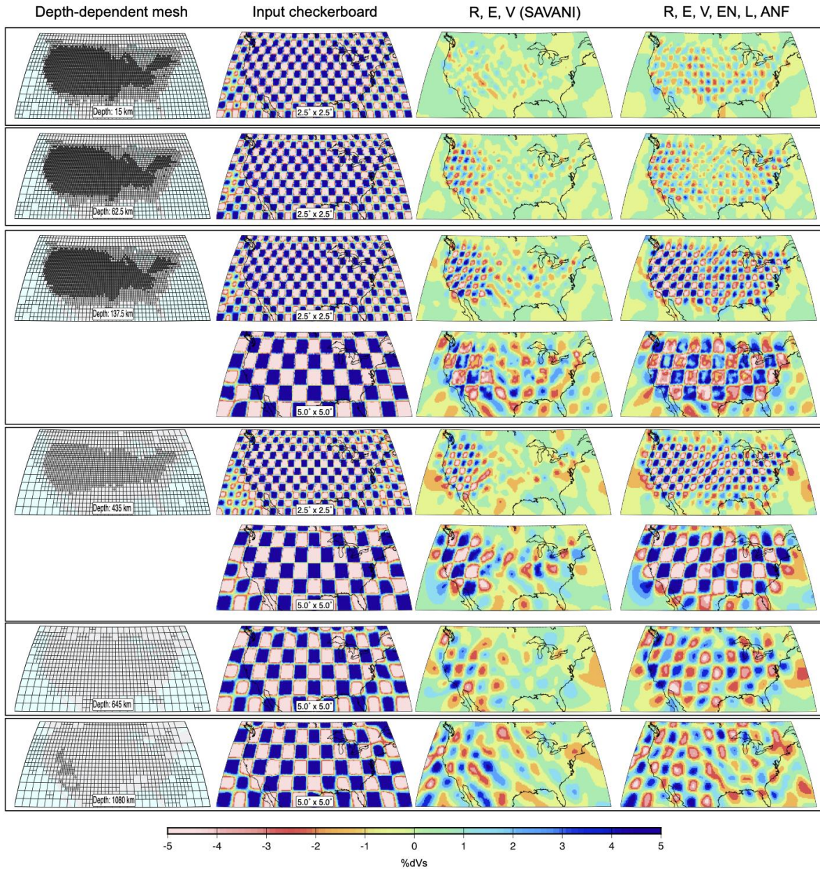
Figure 3: contiguous US scale checkerboard resolution tests. Labeling is as Figure 2 above.
