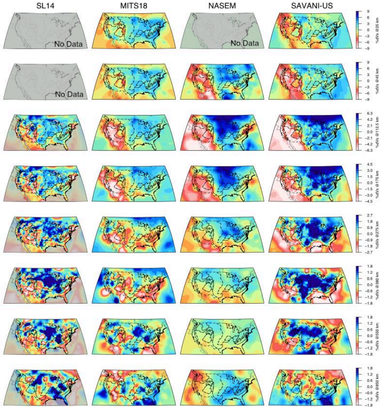
Figure 6: Map view comparison of regional US velocity models. Each column represents one model and each row is a depth slice with a common color scale indicated on the right. Left-hand column is SL14 (Schmandt & Lin, 2014), second from left is MITS18 (Golos et al. , 2018), third from left is NASEM (Clouzet et al. , 2018), and the right-hand column is SAVANI-US (this study).
