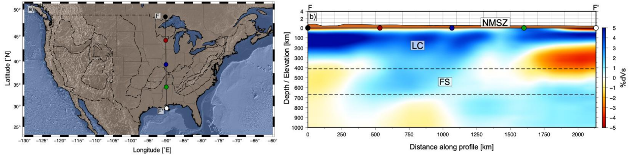
Figure 9: Cross-section through the New Madrid Seismic Zone. Panel (a) is the location map and panel (b) is the north to south cross-section. Labels indicate major features: Laurentia Craton (LC), New Madrid Seismic Zone (NMSZ), and Farallon Slab (FS).
