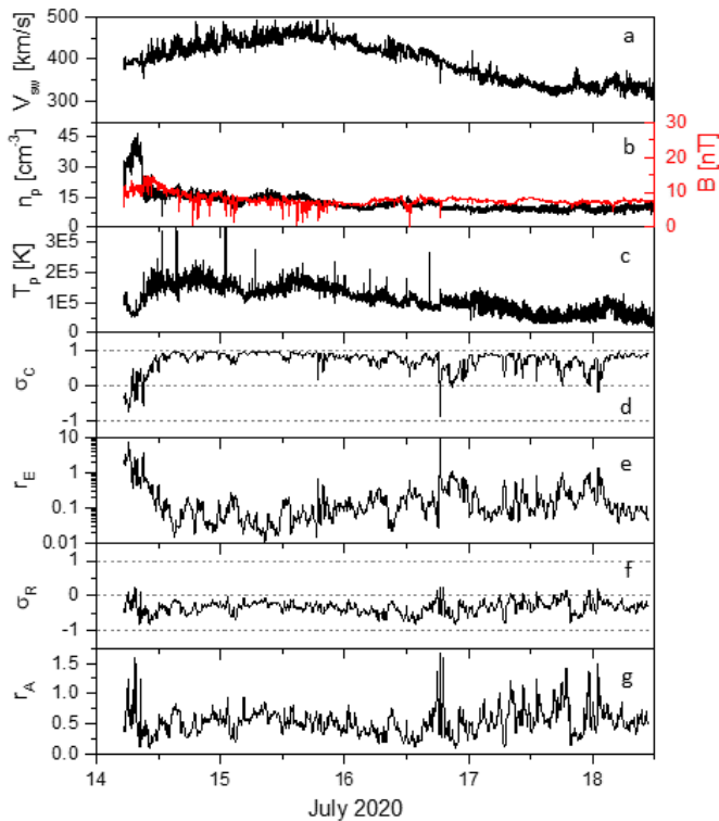
Fig. 2. Time series of plasma and other relevant parameters characterizing Alfvénicity in the slow wind stream observed by Solar Orbiter at a heliocentric distance of 0.64 AU: solar wind speed, V_{sw} [km/s] (a); proton number density, n_p [ \text{cm}^{-3} ] (black) and magnetic field magnitude, B (red) (b); proton temperature, T_p [K] (c); the normalized cross-helicity, \sigma_c (d); the Elsässer ratio, r_E (e); the normalized residual energy, \sigma_R (f); and the Alfvén ratio, r_A (g). The derived quantities are computed at 30 min scale.
