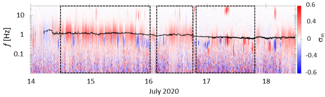
Fig. 7. Spectrogram of the normalized magnetic helicity, \sigma_m . The dashed boxes are the same identified in Fig. 4. The black line corresponds to the proton gyro-frequency.
