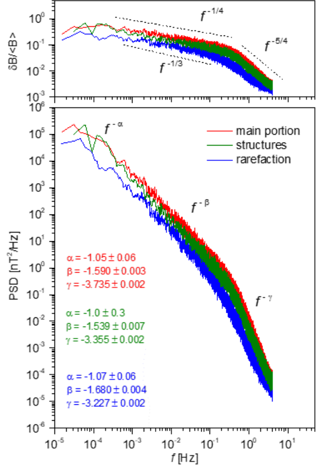
Fig. 6. Top panel: Normalized Power Spectral Density (PSD), \delta B/\langle B \rangle , derived as explained in the text, for the main portion of the stream (red), for the rarefaction region (blue), and for the intermediate region (green). The dashed lines correspond to the Kolmogorov scaling ( \delta B(f) \sim f^{-1/3} ) and to the Kraichnan scaling ( \delta B(f) \sim f^{-1/4} ), along with a scaling \delta B(f) \sim f^{-5/4} corresponding to P(f) \sim f^{-7/2} , according to the normalization described in the text. Bottom panel: PSD of the trace of magnetic field components for the three identified regions as in the top panel. The slopes of the three frequency regimes are indicated with the same color code of the different portions of the stream and are computed over the following frequency ranges: f < 3 \cdot 10^{-4} Hz, 2 \cdot 10^{-3} < f < 10^{-1} Hz and 2 \cdot 10^{-1} < f < 2 Hz.
