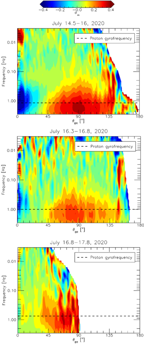
Fig. 8. Scalogram of the normalized magnetic helicity, \sigma_m (color map), with respect to the angle, \theta_{BR} , between the magnetic field and the radial direction. From top to bottom: main portion of the stream, intermediate region and rarefaction region. The dashed line in each plot corresponds to the proton gyrofrequency in the s/c frame.
