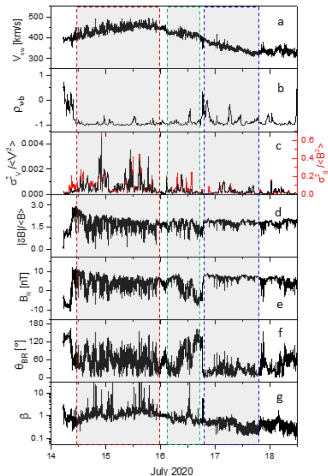
Fig. 4. Time series of relevant parameters: solar wind speed, V_{sw} [km/s] (a); v - b correlation coefficient, \rho_{vb} (b), computed at 30 min scale (b); V and B variances normalized to the square of their respective mean fields, \sigma_V^2 / \langle V^2 \rangle (black) and \sigma_B^2 / \langle B^2 \rangle (red) (c); magnetic field vector displacement, |\delta \mathbf{B}| / \langle B \rangle (d); radial component, B_R [nT], in RTN coordinate system (e); angle between the magnetic field direction and the radial direction, \theta_{BR} (f); and plasma beta, \beta (g). The red and blue boxes identify the main portion of the stream and the rarefaction region, respectively. The green box identifies a region characterized by the presences of structures, that will be studied in detail in Section 3.4.
