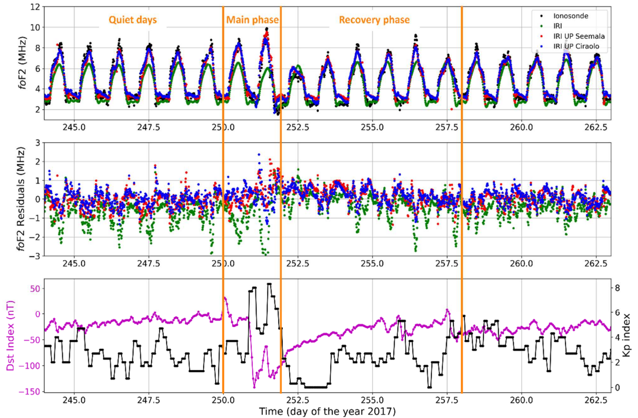
Figure 5. (top panel) foF2 time series measured by (black dots) Hermanus ionosonde, (green dots) modeled by IRI, (red dots) modeled by IRI UP Seemala , and (blue dots) modeled by IRI UP Ciralo for the period 1-19 September 2017. (middle panel) Corresponding time series of residuals between modeled and measured foF2 values. (bottom panel) K_p and D_{st} geomagnetic indices time series, in black and magenta, respectively. Vertical lines define the quiet, main phase, and recovery phase time windows.
