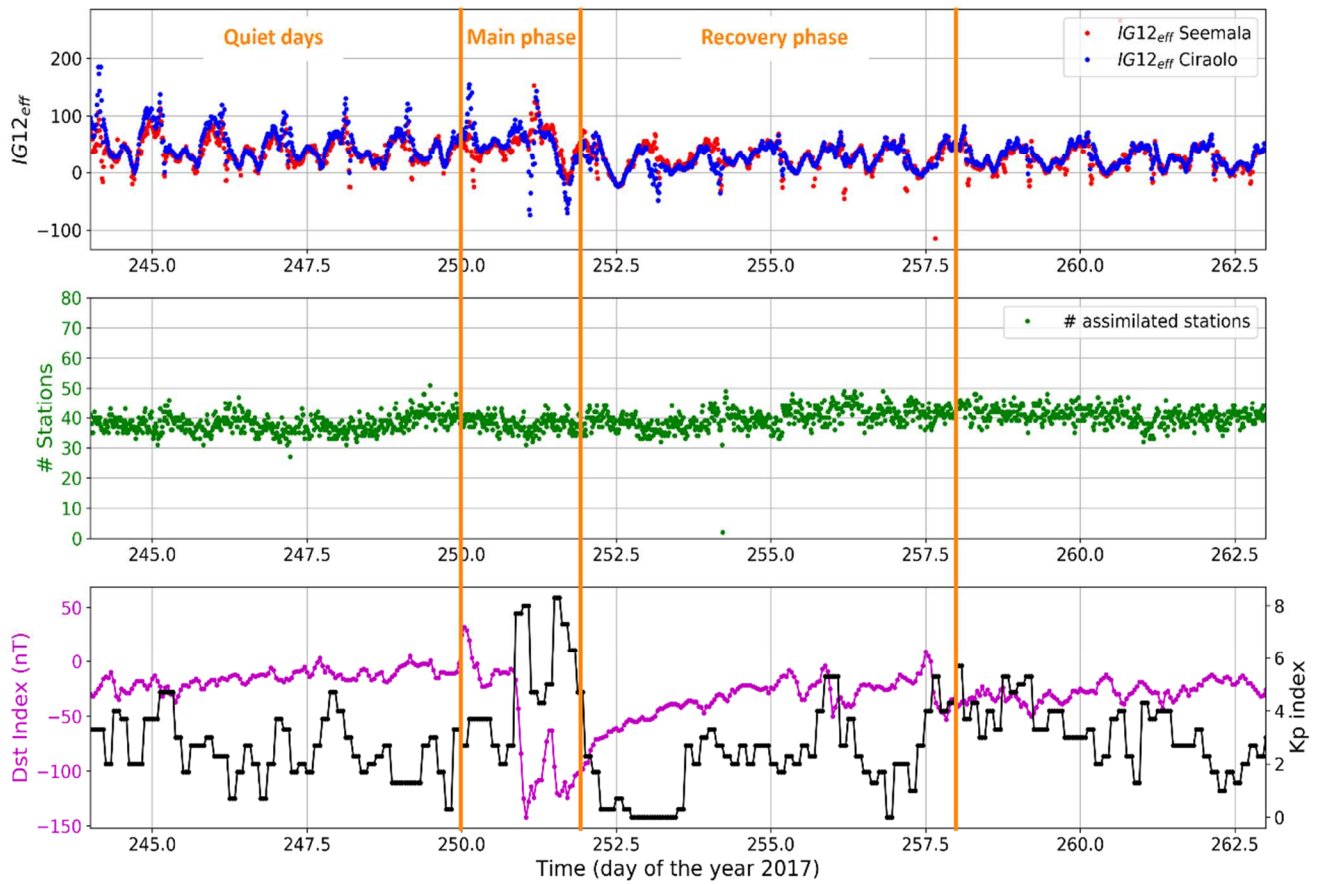
Figure 4. (top panel) IG_{12\text{eff}} time series derived from (red dots) Seemala and (blue dots) Ciraolo vTEC calibration method for the period 1-19 September 2017. (middle panel) Number of assimilated TrigNet GNSS receivers. (bottom panel) K_p and D_{st} geomagnetic indices time series, in black and magenta, respectively. Vertical lines define the quiet, main phase, and recovery phase time windows.
