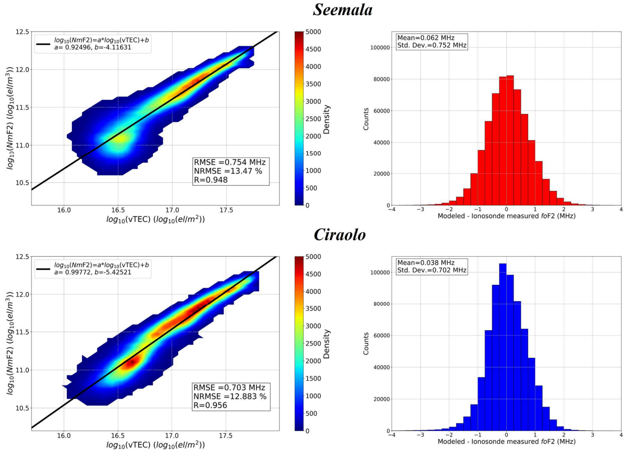
Figure 1. (left panels) Two-dimensional density plot of \log_{10}NmF2 vs \log_{10}vTEC with the corresponding fitting linear function (solid black line). (right panels) Histogram of corresponding residuals between modeled and measured foF2 values. Top panels concern results obtained with Seemala calibration method (adapted from Figure 2 of SWj_paper ), bottom panels concern results obtained with Ciraolo calibration method.
