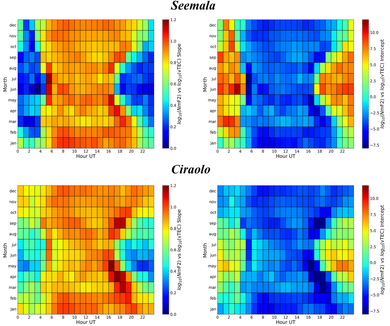
Figure 2. Matrices of the linear fitting coefficients a_{NmF2} (left panels) and b_{NmF2} (right panels) calculated by means of the linear regression (1) for measurements taken at a specific UT hour ( x axis), for a specific month ( y axis), after applying the Seemala's vTEC calibration (top panels, adapted from Figure 3 of SWj_paper ), and the Ciraolo's vTEC calibration (bottom panels).
