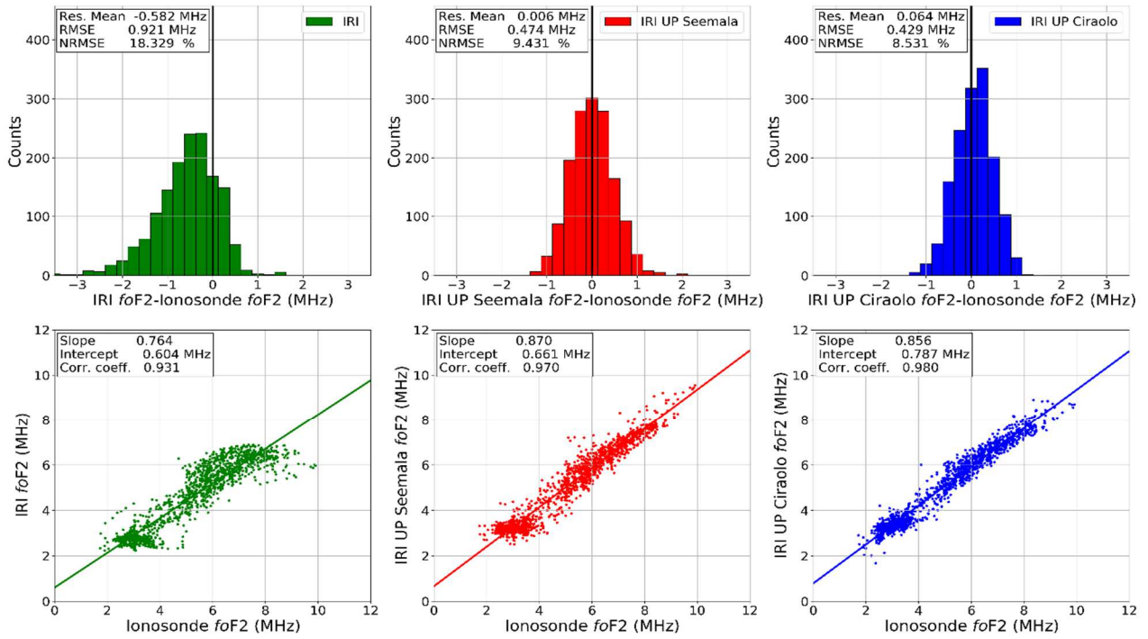
Figure 6. (top panels) Histograms of residuals shown in the middle panel of Figure 5, for (green) IRI, (red) IRI UP Seemala , and (blue) IRI UP Ciraolo , for the period 1-19 September 2017. The residuals mean, RMSE, and NRMSE are shown in the upper left corner of each histogram. (bottom panels) Corresponding scatterplots of modeled and measured foF2 values for IRI, IRI UP Seemala , and IRI UP Ciraolo ; straight solid lines are the best fitting linear functions whose slope and intercept values are shown in the upper left corner of each scatterplot, along with the Pearson correlation coefficient.
