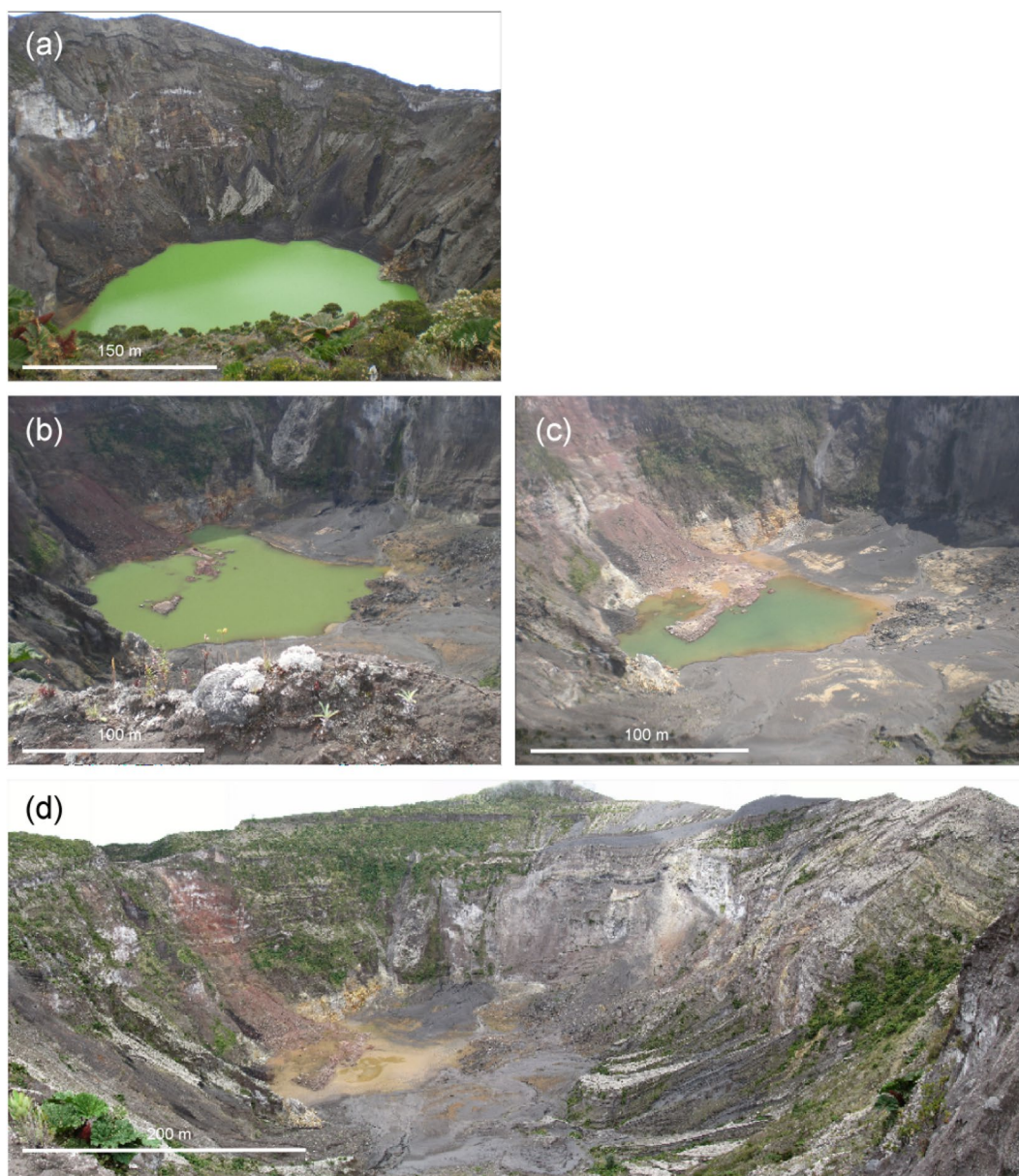
Fig. 2 View of the summit crater lake within the “Cráter Activo” of Irazú in April 2007 ( a from the south), December 2009 ( b from the north), March 2010 ( c from the north), and May 2010 ( d , from the north), showing a progressive reduction of the lake level. Pictures by D. Rouwet ( a, b, c ) and R. Mora-Amador ( d )
