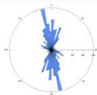
Rift related lineament
