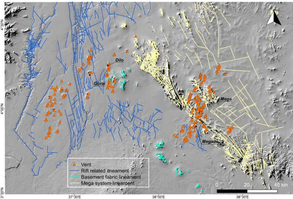
Basement fabric lineament
