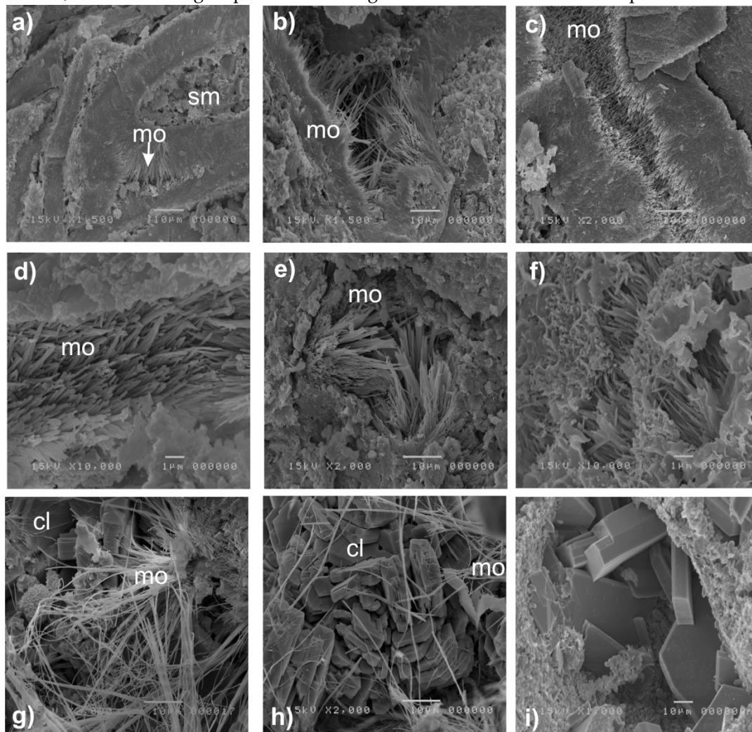
Figure 7. B-SEM (Back Scatter Electron Microscope) images of selected zeolite-bearing samples. (a) Incipient dissolution of the cusped shards to mordenite in aggregating crystals, sample E1b; (b) and (c) from volcanic glass dissolution nucleated and growth acicular crystals of mordenite with characteristic “intertwined bundles”, sample E1a; (d) shards altered to acicular mordenite, sample E1b; (e) and (f) micro-cavities filled by acicular aggregating mordenite crystals, sample E1b; (g) mordenite with acicular shape grown on the glassy component, sample F3; (h) small cavity filled by clinoptilolite laths on which rare acicular mordenites occur, sample F2; (i) cavity filled by euhedral clinoptilolite, F1a.
