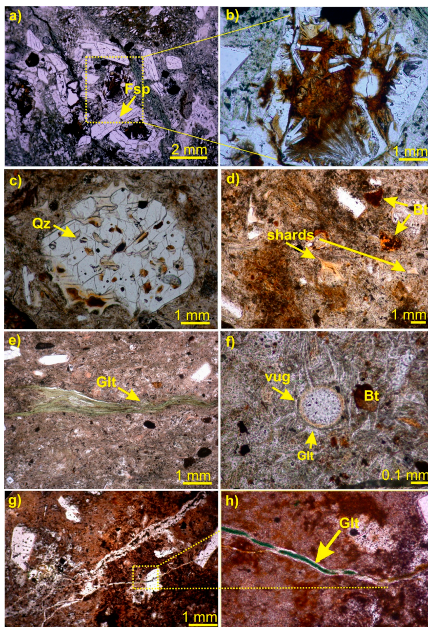
Figure 5. Microphotographs showing textural and mineralogical features of selected samples under OM: (a) and (b) Feldspar with alteration signs in I1 sample under plane polarized light; (c) rounded quartz with several micro-voids in H2 sample, under cross polarized light; (d) cusped glassy y-shaped shards partially transformed into clinoptilolite aggregate in the H3 altered epiclastites under cross polarized light; (e) glauconite in ashy sample E1a, under plane polarized light; (f) vugs filled by clinoptilolite crystals in E2 sample, under plane polarized light; (g) glauconite and (h) its particular grown in veins crossing the reddish matrix of the sample E1d, under plane polarized light. Note the vein-filling or fluid-mimicking aspect of glauconite mineralization in (e) and (h). Abbreviations: Fsp: feldspar; Qz: quartz; Glt: glauconite; Bt: biotite.
