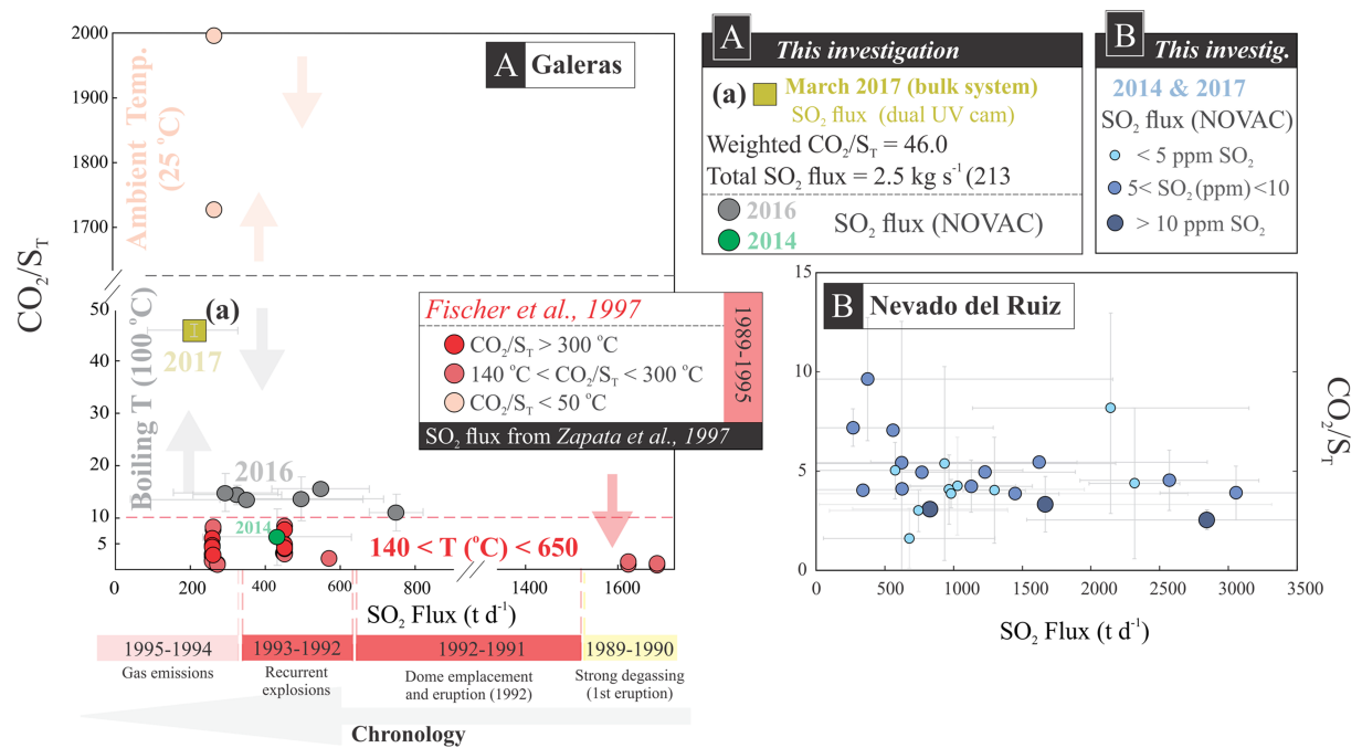
Figure 9. (a) Galeras: CO 2 /S T versus SO 2 flux (t/day) from 1989 to 1995 (CO 2 /S T from Fischer et al., 1997, and SO 2 flux data from Zapata et al., 1997), in different shades of red representing different gas temperature ranges. February–July 2016 data in gray (SO 2 flux records from NOVAC) and 2017 data in olive drab square (SO 2 flux estimates from dual UV camera system); 1989–1995 activity chronology at Galeras is given below (a) (from Zapata et al., 1997). (b) Nevado del Ruiz: CO 2 /S T versus SO 2 flux (t/day), in blue. Categories I to III are distinguishable by different circle sizes, and darker tones of blue for higher SO 2 concentrations.
