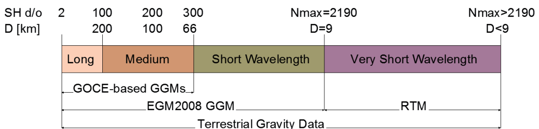
Fig. 1 - The spectral enhancement method (SEM) principle (Zaki et al. , 2018).
