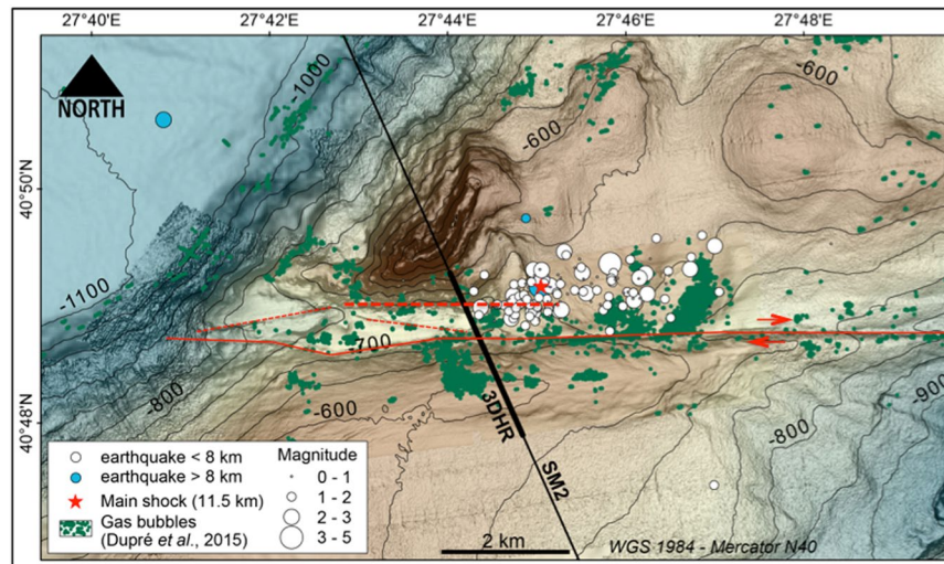
Figure 4. Epicenter locations for the aftershocks that followed the M 5.1 earthquake of July 25, 2011, superimposed on a high-resolution bathymetric grid derived from a combination of near-seafloor AUV data 37 and on an unpublished, bathymetric grid having a resolution of 10 m, based on data collected in 2014 during the Marsite cruise of R/V Pourquoi pas?. White and blue dots are respectively epicenters within and below the sedimentary basin. Green dots indicate the location of the gas emission that were acoustically detected 22 in 2009, using the multibeam echosounder EM302 of R/V Le Suroit. Note that there is no clear overlap between the seismicity (from 2011) and seafloor gas emissions (detected in 2009), e.g. there is no direct evidence that the ultra-shallow aftershocks of 2011 directly induced gas emissions in the water column. Thin black line indicates the track of the seismic section displayed in Fig. 5. The thickened segment represents the location of the 3D, High-Resolution seismic image shown in Fig. 6. The continuous red line indicates the trace of the right-lateral, strike-slip, Main Marmara Fault. Red dotted lines show secondary faults indicating the complexity of the fault network linked to the MMF. The thicker, east-west oriented, dotted line is also shown in the seismic section displayed in Fig. 5. Image created with Arc-GIS, version v3.0.
