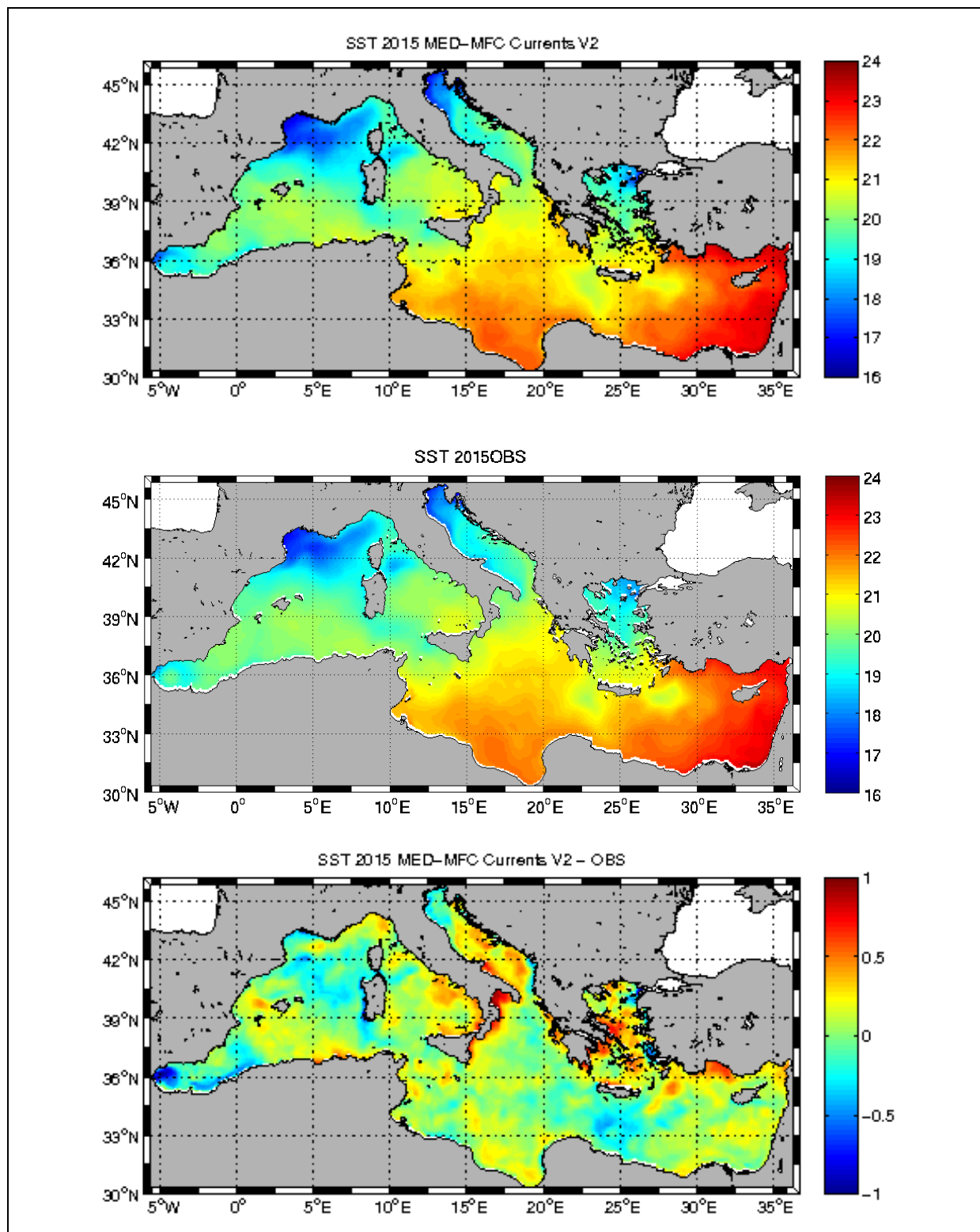
Figure 16: Maps of mean annual (2015) SST computed for V2 system (top), satellite observations (middle) and difference between model and observations (bottom).
