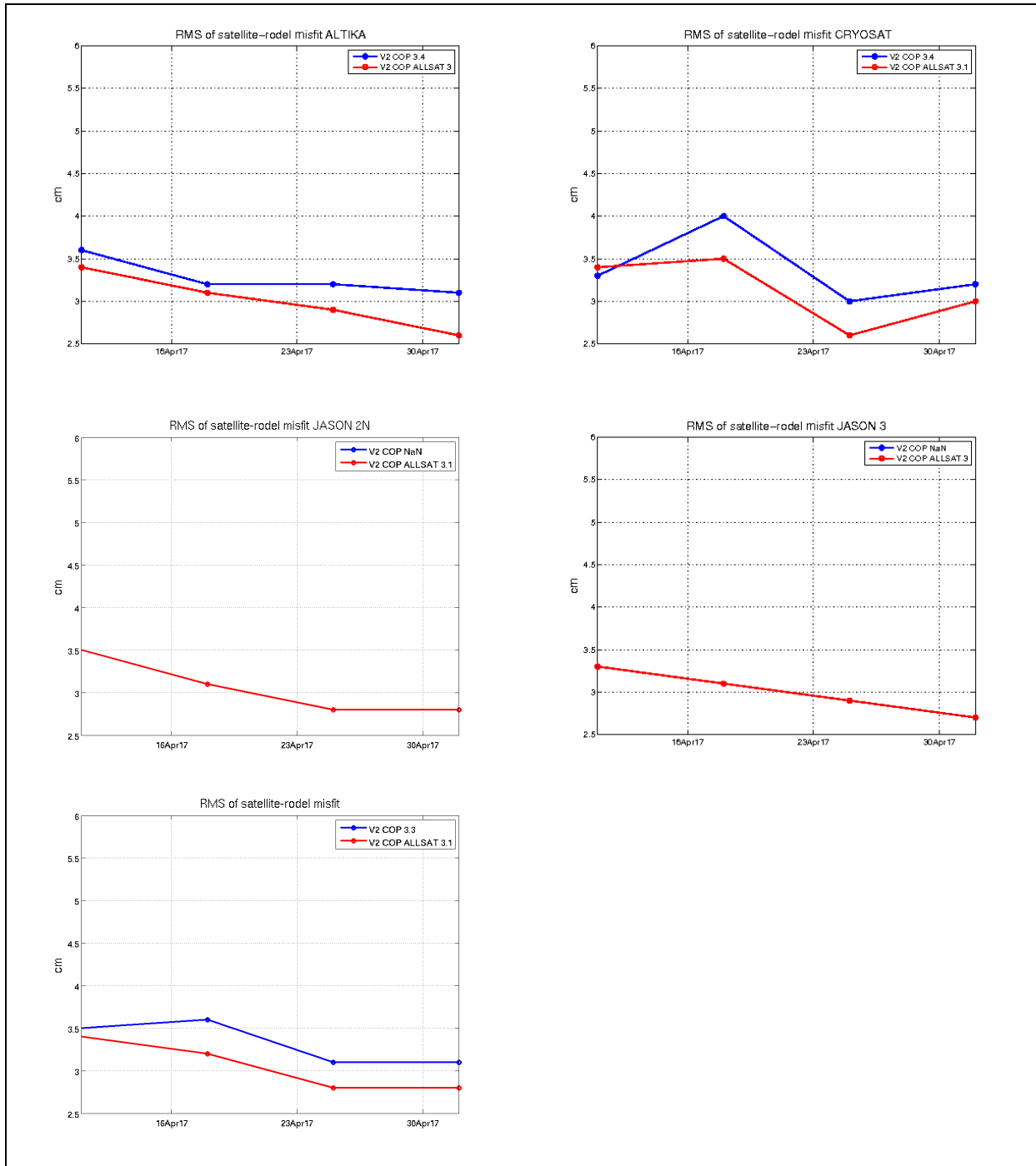
Figure 23 Weekly RMS misfit of satellite-model along SLA data track for Altika (panel top-left), for Cryosat (panel top-right), for Jason2N (panel center-left), for Jason3 (panel center-right), and for all the satellites (panel bottom-left) (SL-CLASS4-RMS).
