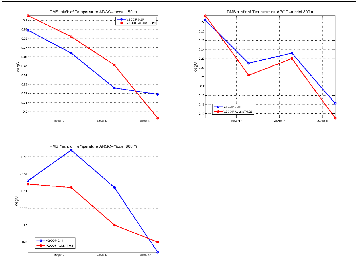
Figure 21: RMS misfit of temperature ARGO-Model at 8, 30, 150, 300 and 600 m (T-CLASS4-RMS_DEPTH)
