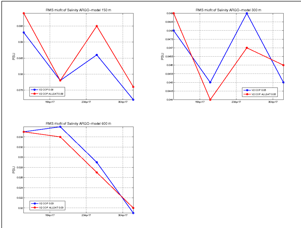
Figure 22: RMS misfit of salinity ARGO-Model at 8, 30, 150, 300 and 600 m (S-CLASS4-RMS_DEPTH)
