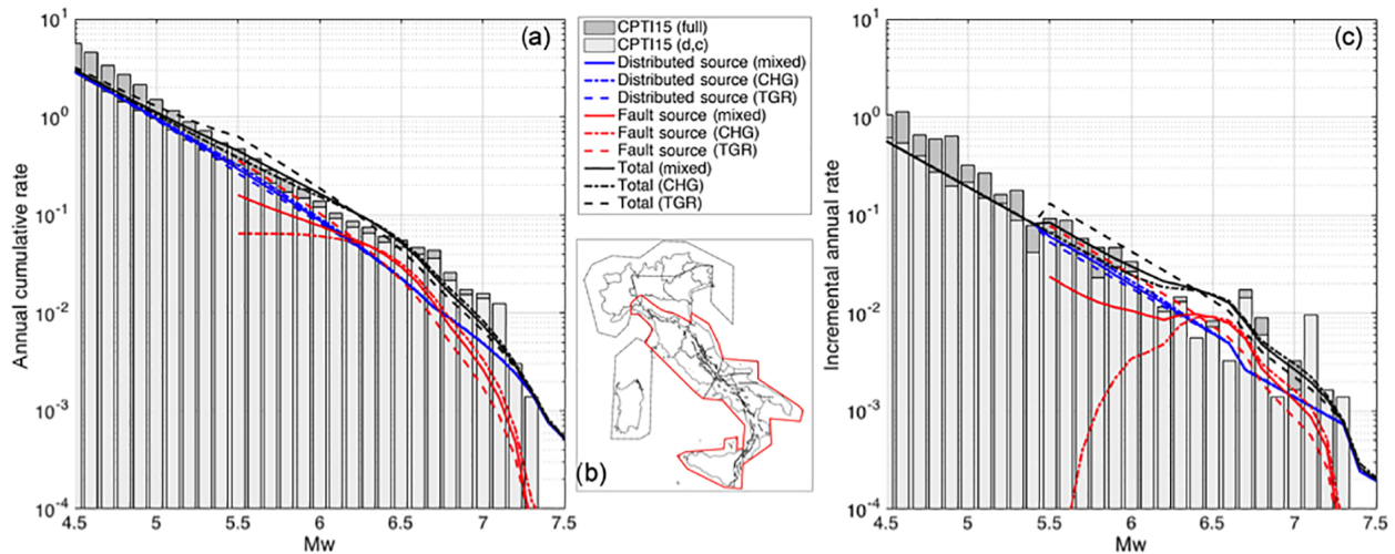
Figure 8. (a) Annual cumulative MFD and (c) incremental annual MFD computed for the red bounded area in (b). The rates have been computed using (i) the full CPTI15 catalogue; (ii) the declustered and complete catalogue (CPTI15, d , c in the legend) obtained using the completeness magnitude thresholds over different periods of time given by Stucchi et al. (2011) for five large zones; (iii) the distributed sources; (iv) the fault sources; and (v) summing fault and distributed sources (total).
