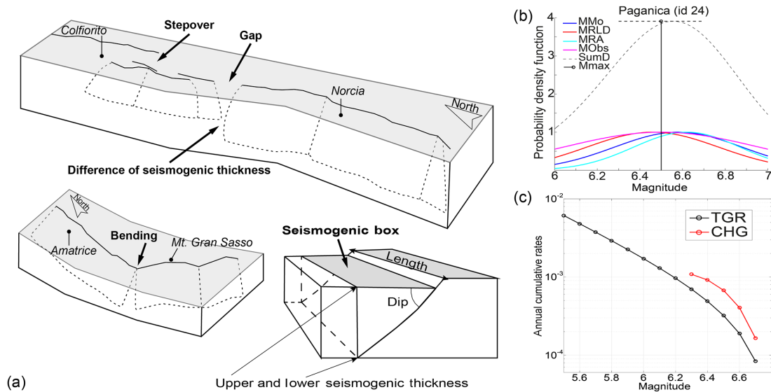
Figure 2. (a) Conceptual model of active faults and segmentation rules adopted to define a fault source and its planar projection, forming a seismogenic box (modified from Boncio et al., 2004). (b) Example of FiSH code output (see Pace et al., 2016, for details) for the Paganica fault source showing the magnitude estimates from empirical relationships and observations, both of which are affected by uncertainties. In this example, four magnitudes are estimated: MMo (blue line), based on the calculated scalar seismic moment ( M_0 ), is from the standard formula (IASPEI, 2005); MRLD (red line) and MRA (cyan line) correspond to estimates based on the maximum subsurface fault length and maximum rupture area from the empirical relationships of Wells and Coppersmith (1994) for length and area respectively; and MObs (magenta line) is the largest observed moment magnitude. The black dashed line represents the summed probability density curve (SumD), the vertical black line represents the central value of the Gaussian fit of the summed probability density curve ( M_{\max} ), and the horizontal black dashed line represents its standard deviation ( \sigma M_{\max} ). The input values that were used to obtain this output are provided in Table 1. (c) Comparison of the magnitude–frequency distributions of the Paganica source, which were obtained using the CHG model (red line) and the TGR model (black line).
