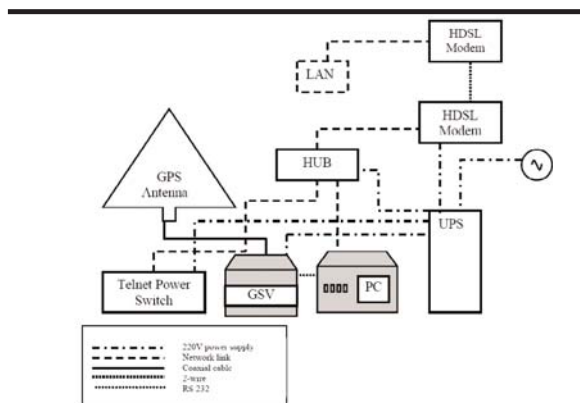
Figure 1. A scheme of a typical GISTM unit configuration adopted in the ISACCO project.
