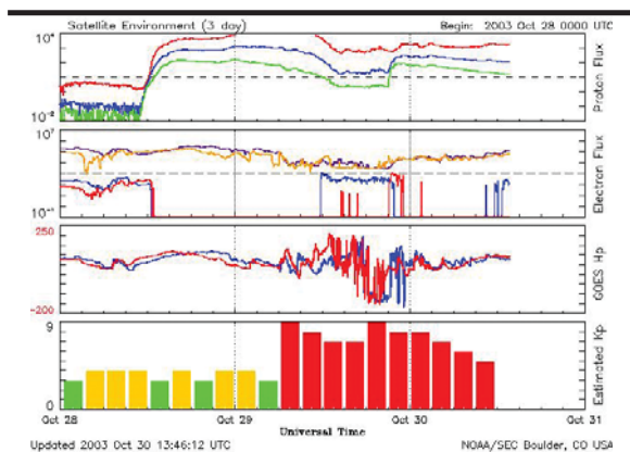
Figure 2. External conditions recorded by the GOES satellites during late October 2003.
