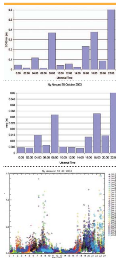
Figure 4. Correlation of 3D errors and RMS residuals (top and middle) with phase scintillation occurrence (bottom) at Ny Alesund on 30th October 2003
