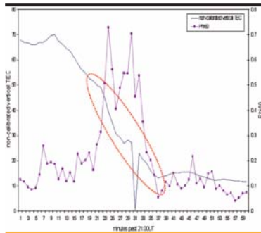
Figure 3. Temporal behaviour of the TEC and 60 seconds \sigma_{\phi} (Phi60) recorded at Ny Alesund (link to PRN 31) between 21 & 22 UT on Oct. 30, 2003.
