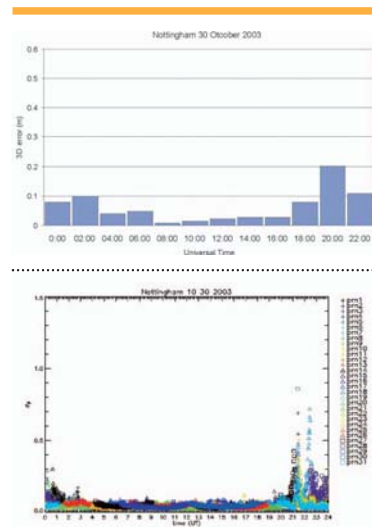
Figure 6. Correlation of 3D errors (top) and phase scintillation occurrence (bottom) at Nottingham on 30th October 2003
