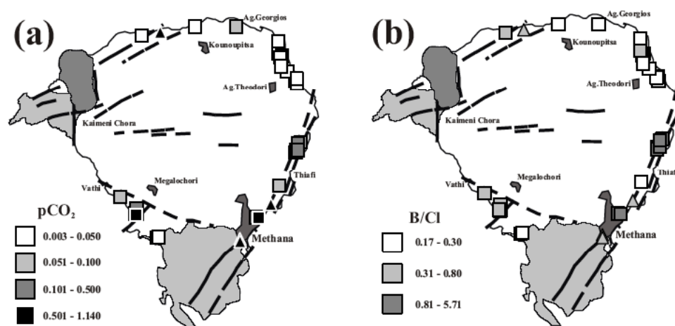
Figure 6 - Distribution of the p\text{CO}_2 (a) and B/Cl (b) values in the groundwaters.
