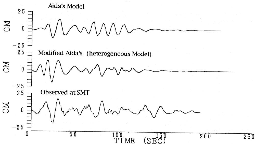
Fig. 16. Comparison of simulated displacements at SMT for the heterogeneous faulting model and the observed one. Top: Aida's model; middle: the heterogeneous faulting model (modified Aida's model); bottom: the observed displacement at SMT.
