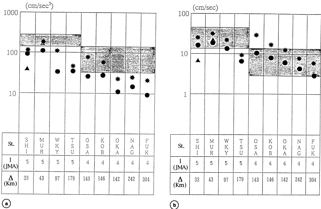
Fig. 17a,b. Comparison of peak ground accelerations (a) and velocities (b) of simulated ground motions to those estimated from the seismic intensities (JMA). Solid circles, triangles, and star marks are the peak values of the simulated ground motions for Aida's, Ando's, and the heterogeneous (modified Aida's) models, respectively. Shadows show the ranges of peak acceleration and velocity empirically evaluated from the JMA intensities.
