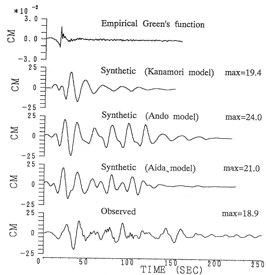
Fig. 12. Comparison of simulated displacements at WKY for three fault models (Kanamori's, Ando's and Aida's) and the observed displacement at SMT. The top trace is the EW displacement record at WKY from the 1991 Shirahama-Oki earthquake ( M_{JMA} = 5.1 ) used as the empirical Green's function. All traces are band-pass-filtered between 0.05 and 0.5 Hz.
