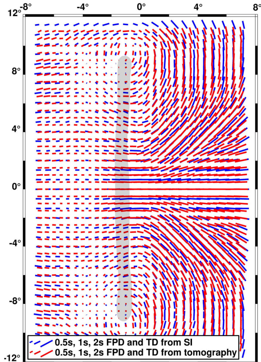
Figure 7. Direct comparison of both shear wave splitting measurements with the grey transparent shape representing the outline of the slab at 150 km depth (Fig. 1a). Marked with red are the splitting parameters restored from the optimal depth dependent shear wave anisotropy model shown in Fig. 5 within the grid of the model. In blue are the splitting parameters from sinusoidal curve fitting (Fig. 2) at each station.
