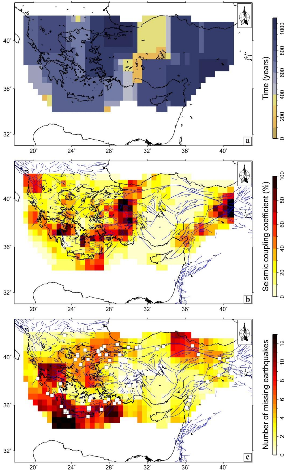
Figure 9. a) Spatial pattern of temporal duration of the M5C catalog. b) Spatial pattern of the seismic coupling coefficient coupling (SCC). c) Missing earthquakes over a time interval of 400 years.
