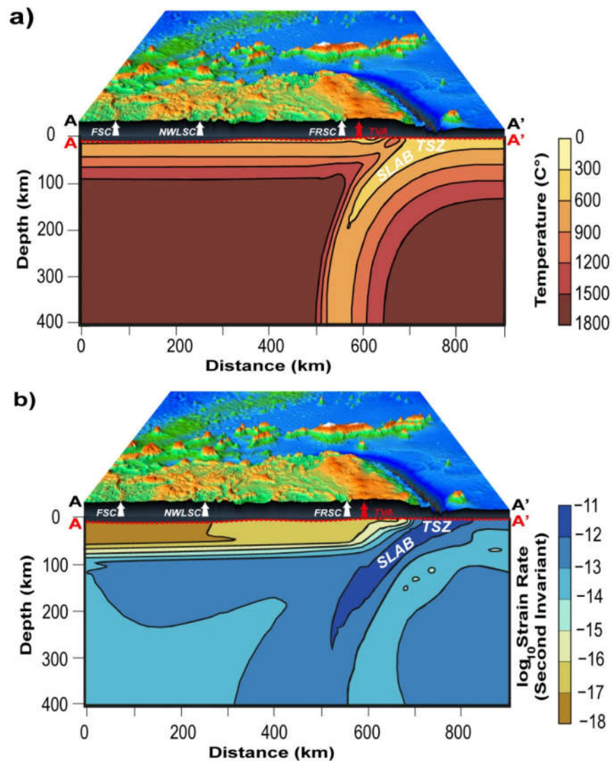
Figure 8. Conceptual models showing the regional bathymetry of the Northern Lau Basin: (a) the distribution of the temperature in the mantle; (b) the second invariant of the strain rate, both predicted by our numerical model. The 3D bathymetry was created using the open source software 3DEM (visualization software created by Richard Horne, USGS, http://www.hangsim.com/3dem/ , accessed on 1 July 2021). Black line A–A': bathymetric profile shown in Figure 2c. Red dashed line A–A': crustal thickens shown in Figure 2c. White arrows indicate the location of the mantle rise below the back arc spreading centers. FSC: Futuna Spreading Center; NWLSC: Northwest Lau Spreading Center; FRSC: Fonualei Rift and Spreading Center; TSZ: Tonga Subduction Zone; TVA: Tonga Volcanic Arc.
