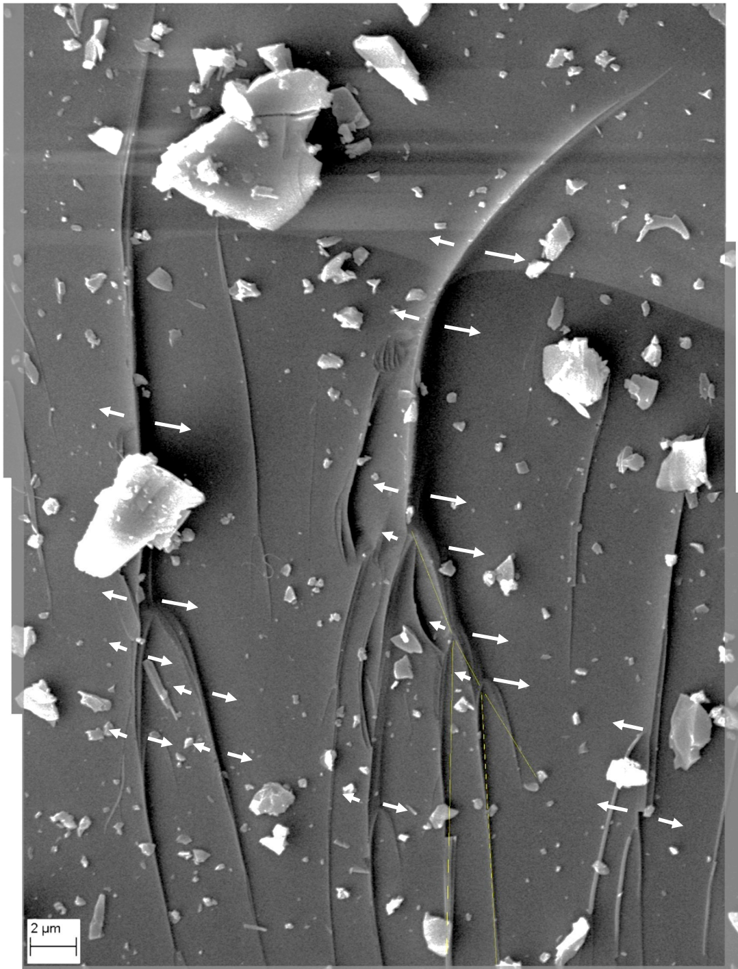
Figure 6. Fractures on the surface of a quartz granule subjected to 100 MPa; the bifurcations show angles of about 27^\circ (taken from the work of Martinelli et al. [5]).
