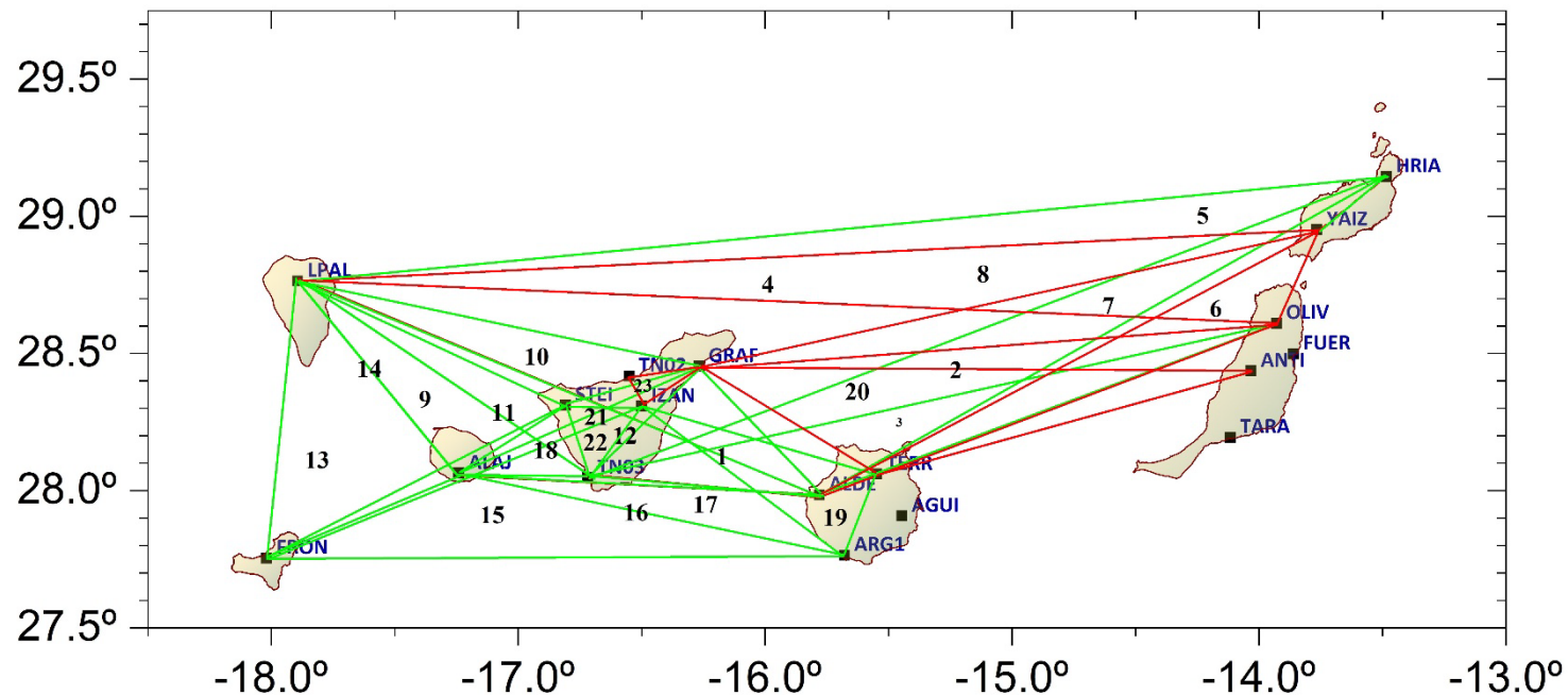
Figure S1. Triangles formed from 3 non-co-linear stations each, for the 23 GNSS stations used in this work (see Table 2). The horizontal strain was subsequently calculated for each triangle's centroid. The colour lines are just to draw a clearness figure.
