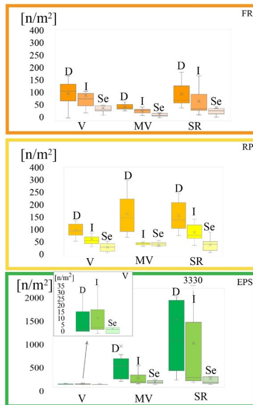
Figure 4. Distribution of FR (orange box on the top), RP (yellow box in the middle) and EPS densities (green box below), expressed in number of items for square meter ( n/m^2 ), per site (SR, MV, V) according to the beach zonal analysis (Dune: D, Intermediate: I, Sea: Se). The enlarged box shows in detail the situation of Viareggio for EPS fraction.
