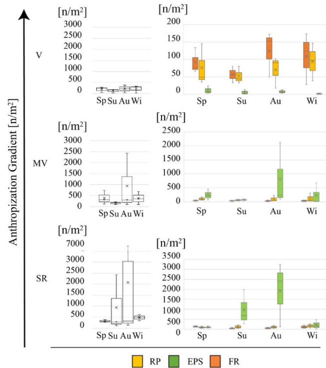
Figure 3. Distribution of MP density, expressed in number of items for square meter ( n/m^2 ) per site (SR, MV, V): considering the 3 MP types together on the left, and separated on the right. (Sp = spring, Su = summer, Au = autumn, Wi = winter).
