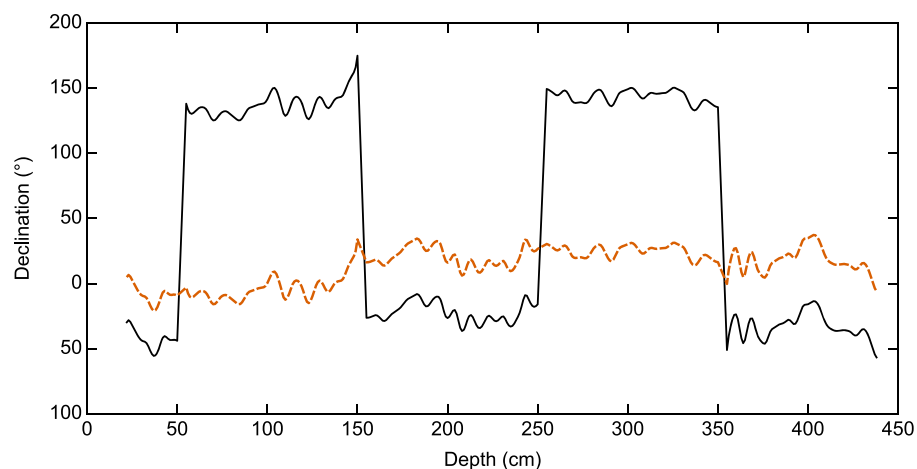
Figure 3. Automatic declination realignment applied to declinations from Core C5 of NEXTDATA cruise AMICA2013 (Margaritelli et al., 2016). Before plotting and processing, the top two and bottom two samples from each core section were removed to exclude artifacts at the extreme ends of the cores. Black solid line: original declinations as calculated by principal component analysis. Orange dashed line: automatically realigned declinations using an absolute declination of 0 and a mean direction from six samples at each core section end.
