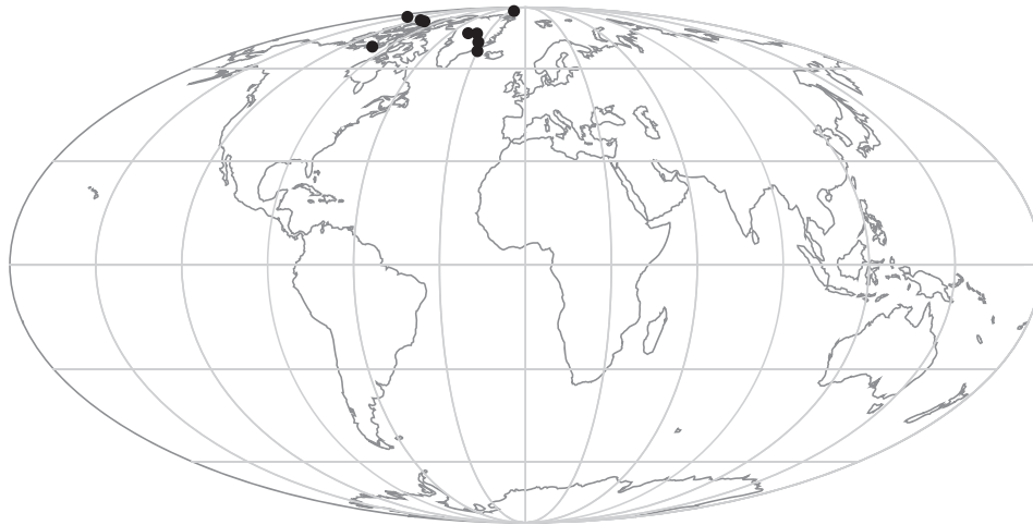
Figure 5. An example of VGP calculation on synthetic data in PuffinPlot. Data were generated for nine sites at different geographic locations, with 10 samples at each site. Sample directions were generated by adding random noise to the direction calculated by the IGRF-12 geomagnetic model for the year 1900. (top) Suite parameter table, giving Fisherian statistics on site and sample directions and VGPs. (middle left) Site parameter table, showing paleomagnetic direction at each site. (middle right) VGP parameter table, showing locations of sites and site VGPs. VGP = virtual geomagnetic poles.
