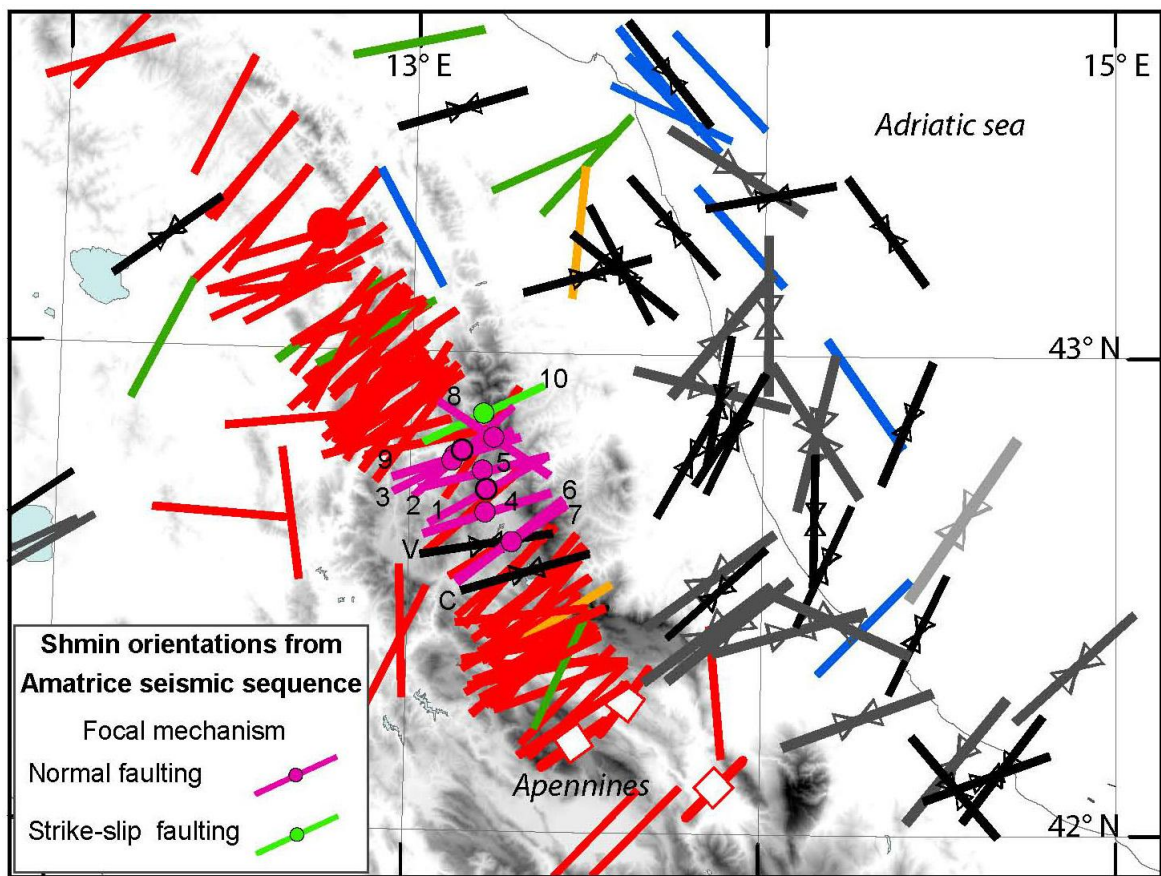
Figure 2. The 2016 Italian stress map and the new minimum horizontal stress ( S_{hmin} ) orientations inferred from the available focal mechanisms of ten earthquakes with M_w \geq 4 [ http://autorcmnt.bo.ingv.it/quicks.html ]. Numbers as in Table 1. Bold circles are the event n. 1 and n. 2 of Figure 1 and Table 1. V and C stand for Varoni and Campotosto wells. See legend in Figure 1.
