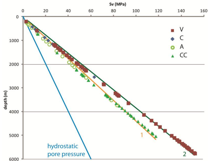
Figure 4. Vertical stress ( S_v ) estimated from sonic log data. 1, trend line of data from the wells in the foredeep (A and CC); 2, is relative to the wells in the Apennine belt (V and C).
