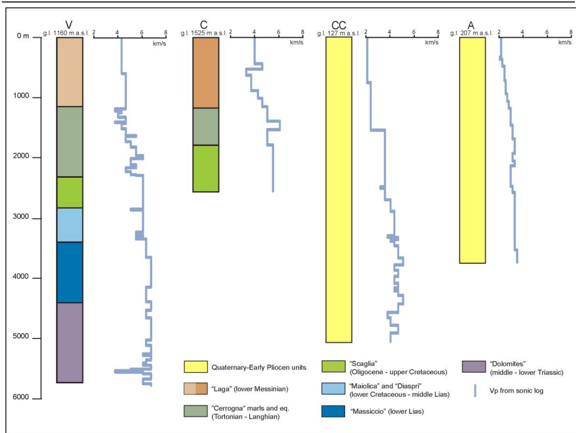
Figure 3. Stratigraphic sequence and P-wave velocity ( V_p ) at depth along V, C, CC, and A wells (see Figure 1 for location) as inferred from sonic log.
