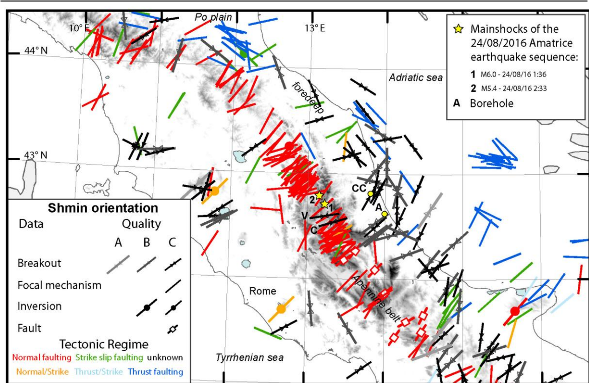
Figure 1. Present-day stress in central Italy. Minimum horizontal stress ( Sh_{min} ) orientations [Montone and Mariucci, 2016] and the two mainshocks of the Amatrice seismic sequence until October 3 rd , 2016 [BSI, 2016]. Normal faulting regime: Sh_{min} = \sigma_3 ; Strike-slip: Sh_{min} = \sigma_3 ; Thrust: Sh_{min} = \sigma_2 . Location of the boreholes analysed in this study: A, Atri; CC, Colle Casone; C, Campotosto; V, Varoni.
